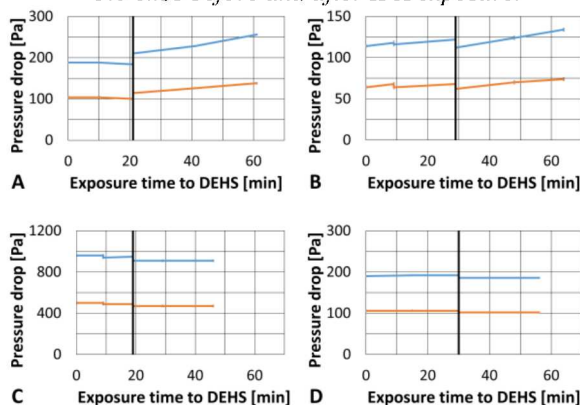
Figure 2. Pressure drop of medium as a function of exposure time to DEHS. At 3.0 cm/s in blue and at 1.7 cm/s in orange.
