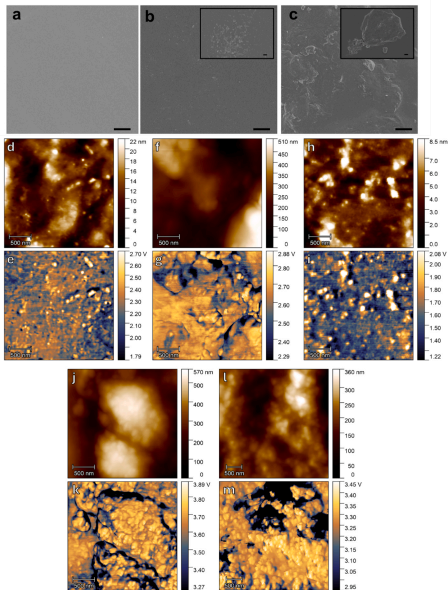
Fig. 4. Scanning electron microscopy of Pristine (a), 2% w/w SB-NPs (b), 5% w/w SB-NPs (c). Atomic force microscopy and corresponding maps of (d-g) pristine, (h-k) 2% w/w SB-NPs, and (l-m) 5% w/w SB-NPs.
