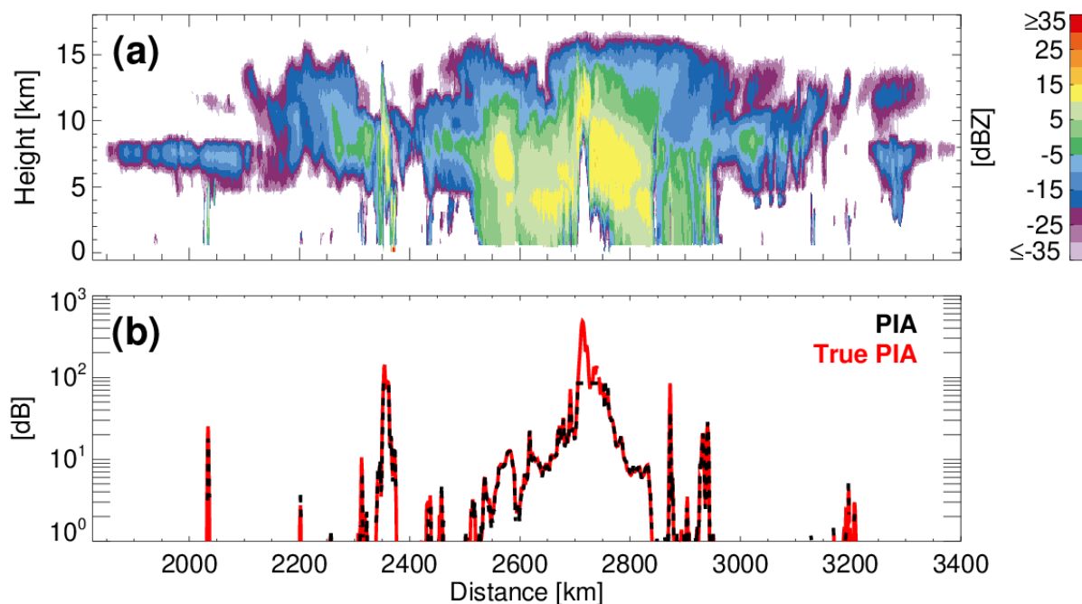
Figure 2. a) The CPR radar reflectivity from the 1825 - 3400 km along-track segment of the Hawaii (tropical) scene, b) the C-PRO estimated (black line) and true (red line) PIA time series from the same segment of the Hawaii scene over the ocean.
