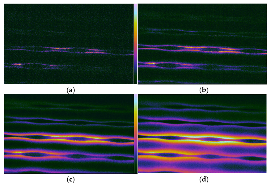
Figure 5. V2 prototype: IR image frames obtained with macrolens after (a) 8 s of excitation; (b) 14 s of excitation; (c) 24 s of excitation; (d) 38 s of excitation.
