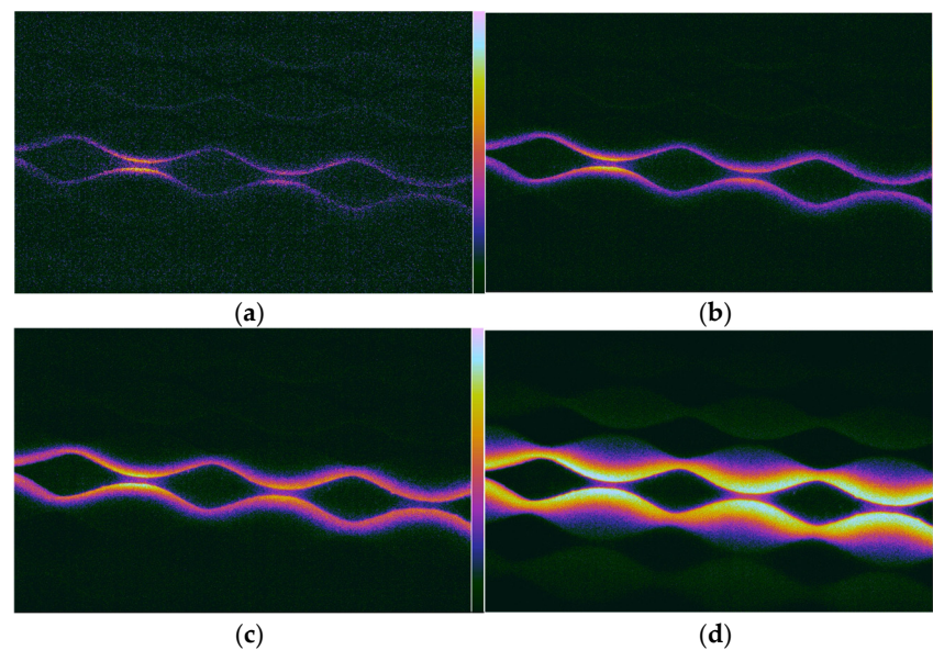
Figure 4. V1 prototype: IR image frames obtained with macrolens after (a) 8 s of excitation; (b) 14 s of excitation; (c) 24 s of excitation; (d) 38 s of excitation.
