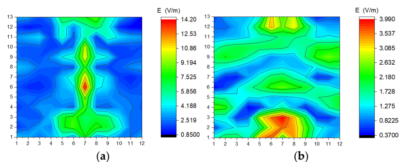
Figure 3. (a) E-field maps at 2 mm distance from the surface of prototype V1: (a) f = 5.65 GHz; S_{21} = -2.065 dB; (b) f = 10.30 GHz; S_{21} = -58.412 dB. In all plots, microstrip lines are vertical.
