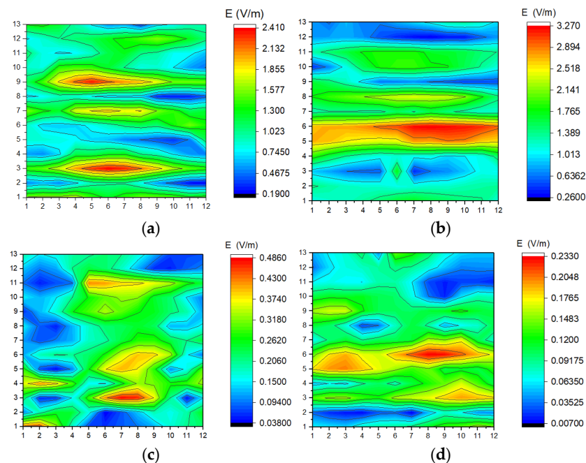
Figure 2. (a) E-field maps at 22 mm distance from the surface of prototype V1: (a) f = 5.65 GHz; S_{21} = -2.065 dB; (b) f = 6.23 GHz; S_{21} = -2.974 dB; (c) f = 10.30 GHz; S_{21} = -58.412 dB; (d) f = 12.49 GHz; S_{21} = -49.99 dB. In all plots, microstrip lines are vertical.
