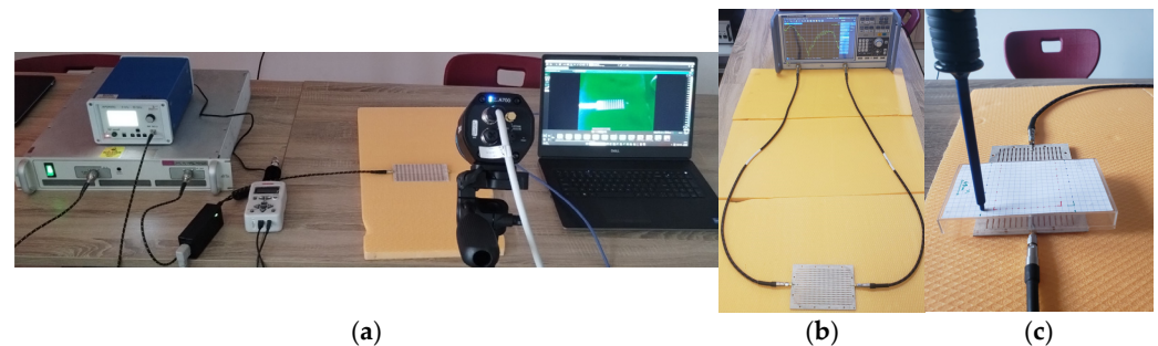
Figure 1. (a) Measurement system setup showing the RF generator, amplifier, power meter, FLIR A400 IR camera and HIS metasurfaces; (b) VNA measurement; (c) the E-field probe and field scanning are shown above the HIS V2 prototype.
