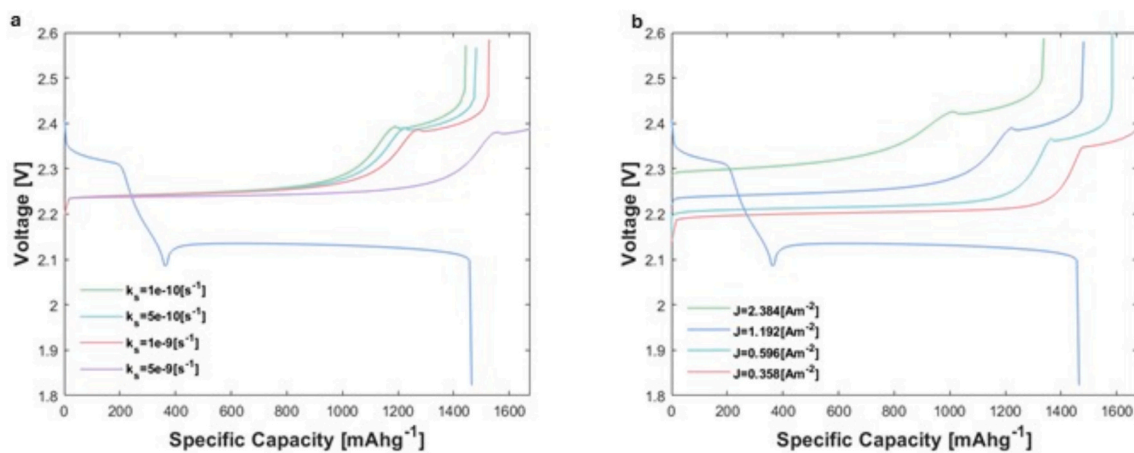
Fig. 4. Parameter analysis on shuttling, using 2nd case of D_{\text{Li}^+} : a) Charge and discharge Voltage profile vs specific capacity at 0.1C with different shuttle constant k_s [\text{s}^{-1}] b) Charge and discharge Voltage profile vs specific capacity at different current intensity, using k_s = 1e-9 [\text{s}^{-1}] .
