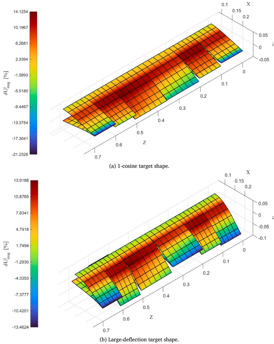
Fig. 18. Original control scheme, V = 0 m/s: final iFEM reconstructed shapes; \delta U_{mag}^j color-map; 10% strain noise.
