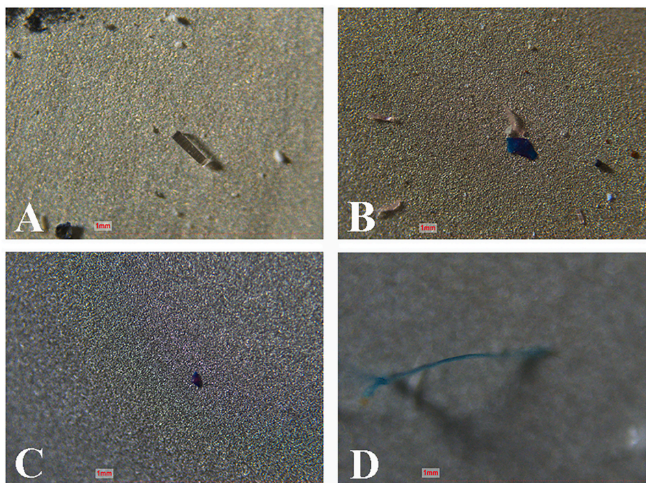
Fig. 3. Images of anthropogenic particles found in Bossea cave waters under microscope. A: transparent polyacrylamide fibre from Rio Roccia Bianca surface watercourse; B: blue copolymer fragment from the overflow; C: blue ethylene vinyl alcohol fragment from Ernestina lake, inside the tourist area of the cave; D: light blue cotton fibre from Polla delle Anatre sampling point, inside the tourist area of the cave.
