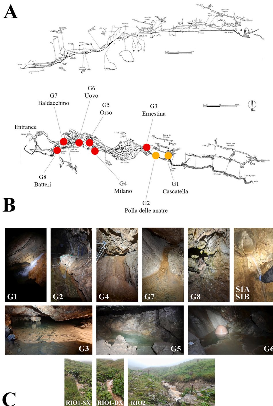
Fig. 2. Sampling points. A,B: Bossea cave surveys. Red circles for water sampling in the tourist area, orange circles for water sampling in the speleological area (Surveys – section (A) and plan (B) - from Elia and Callaris (1988) , modified); C: photos of all sampling points (photo S1A-S1B by E. Lana, all the other photos by V. Balestra).
