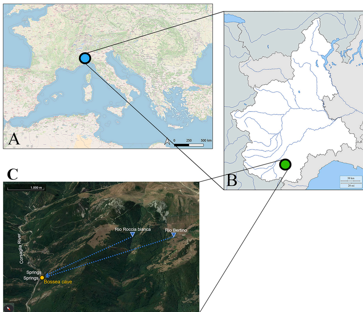
Fig. 1. Study site. A and B: Location of the sampling area (map A created with QGIS Desktop 3.12.1 with GRASS 7.8.2 using OpenStreetMap map, modified - openstreetmap.org/copyright, map B from https://d-maps.com/carte.php?num_car=8256&lang=en , modified); C: Turquoise triangles for the main surface water supply (Rio Roccia bianca and Rio Bertino), orange circle for Bossea cave and springs (Map from https://earth.google.com [accessed: 07/06/2022], modified).
