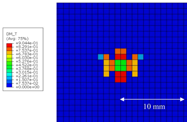
Fig. 13 Tensile matrix-damaged region in the upper surface of the circular plate, 192 Q9-LE3 model
