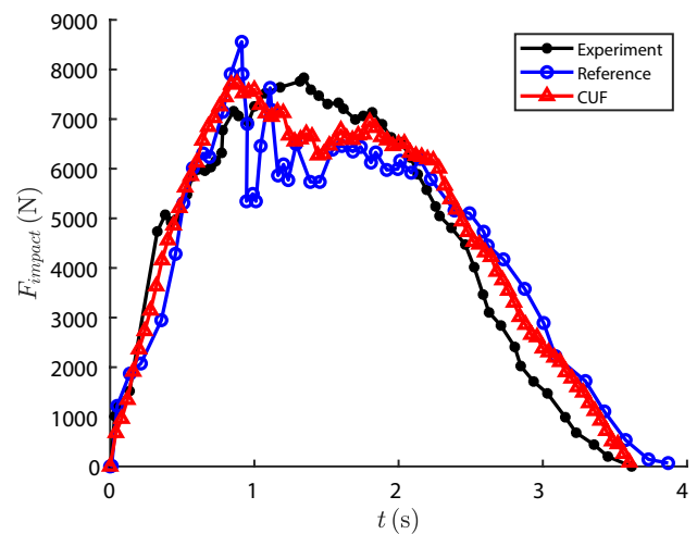
Fig. 16 Force-time response for the rectangular plate. CUF results with 8% smoothing
