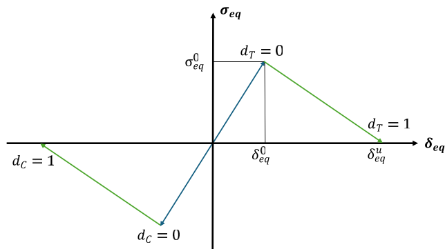
Fig. 1 Bilinear damage evolution
