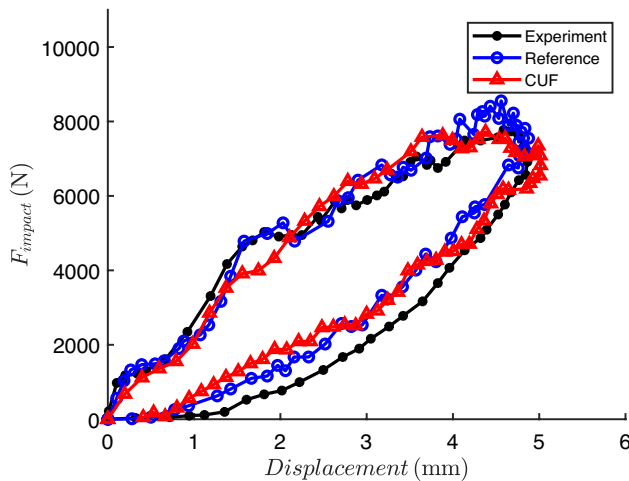
Fig. 17 Force-displacement curve for the rectangular plate. CUF results with 4% smoothing
