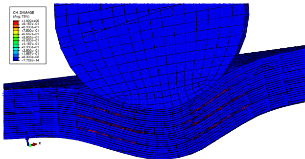
Fig. 20 Delamination at the impact point of the rectangular plate at t = 2.4 ms
