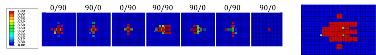
Fig. 14 Left: Delamination at the ply interfaces of the circular plate, ordered through the thickness from the impacted top surface to the bottom face. Right: Delamination envelope through the thickness, 260Q9-LE2 model
