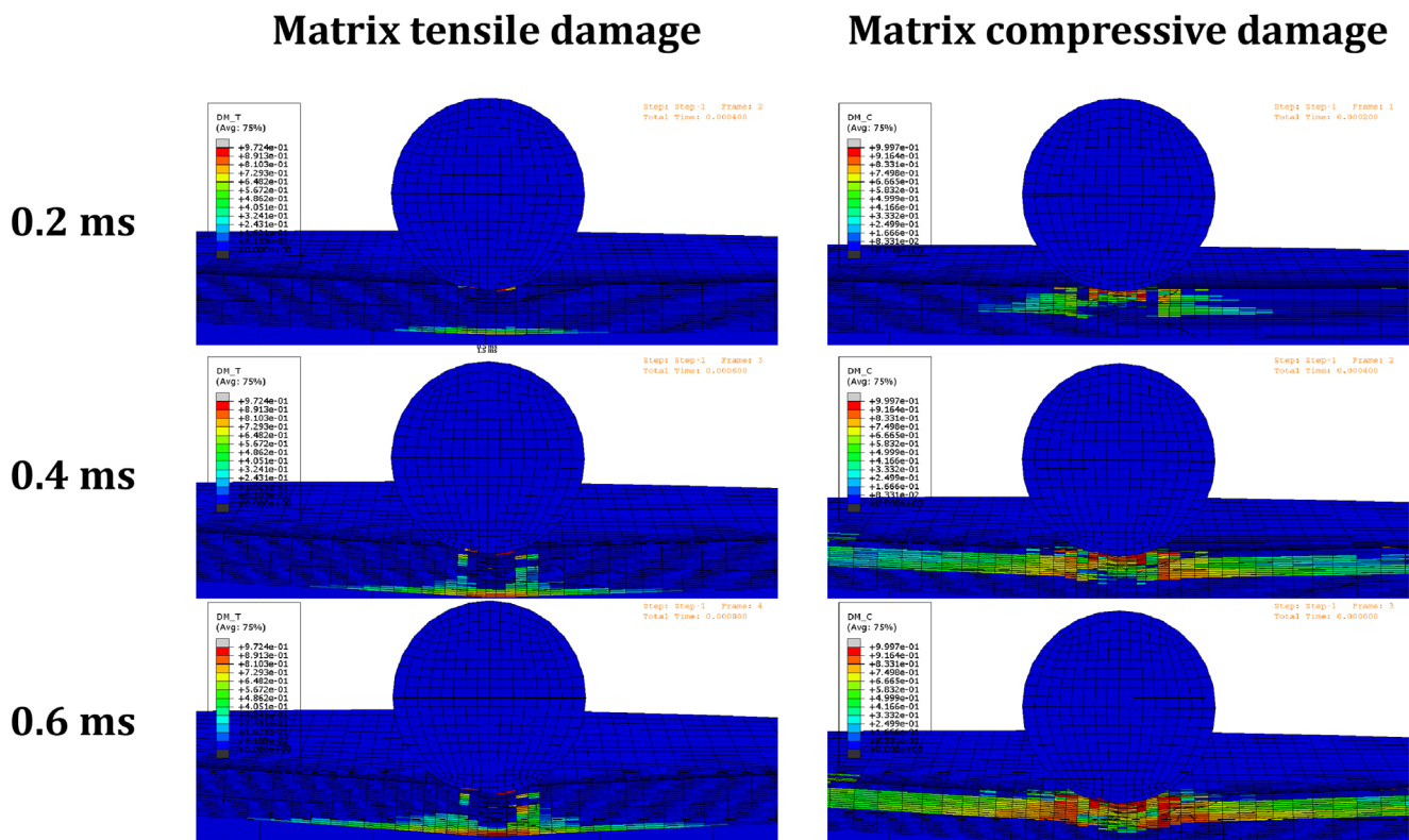
Fig. 19 Damage evolution in the matrix for the rectangular plate
