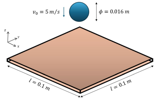
Fig. 4 Elastic impact of the square composite plate
