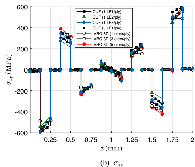
Fig. 5 In-plane stress components through the thickness of the composite plate under elastic impact at (x, y) = (48 \text{ mm}, 48 \text{ mm})
