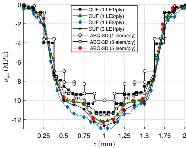
Fig. 6 Transverse shear stress through the thickness of the square plate under elastic impact at (x, y) = (40 \text{ mm}, 40 \text{ mm})
