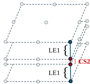
Fig. 2 Two-node cohesive Lagrange through thickness elements (CB2)
