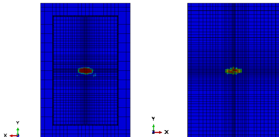
Fig. 20 Delamination at the impact point of the rectangular plate at t = 2.4 ms
