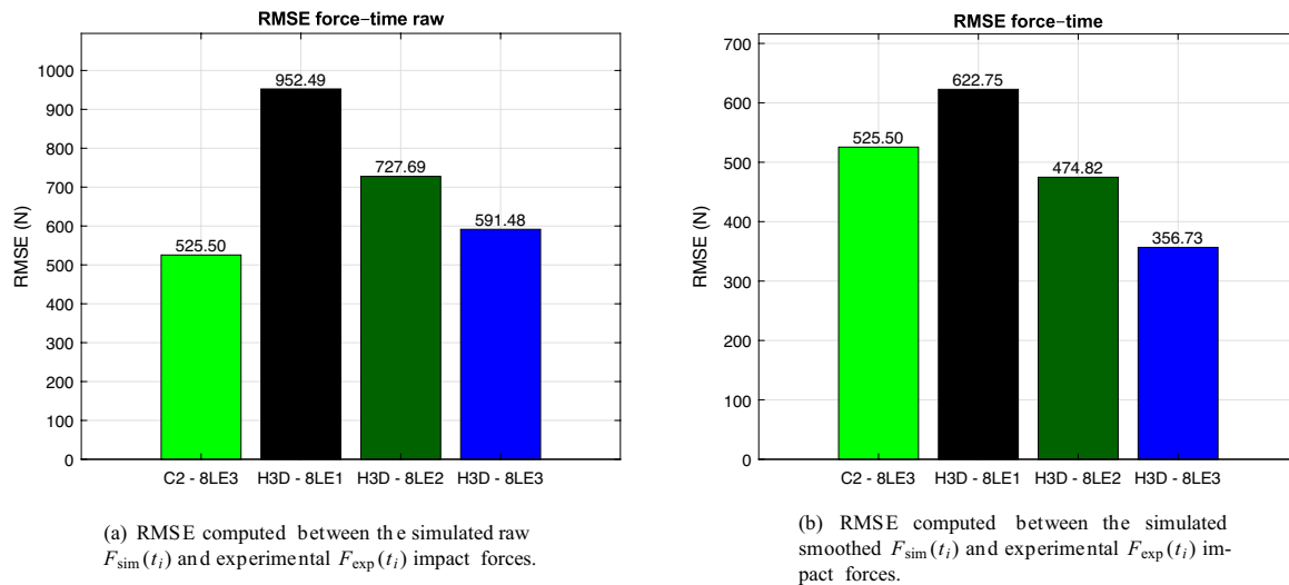
Fig. 11 RMSE of the force-time response for the circular plate. The CUF H-P approach is compared to RMSE values of CODAM2 from [13] (C2)
