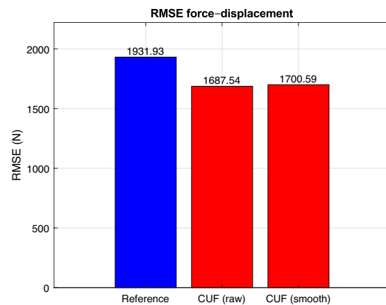
(b) RMSE of the force-displacement response for the rectangular plate, computed between the simulated F_{\text{sim}}(u_i) and experimental F_{\text{exp}}(u_i) impact forces. The CUF approach is compared to reference value from [3].
