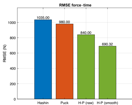
(a) RMSE of the force-time response for the rectangular plate, computed between the simulated F_{\text{sim}}(t_i) and experimental F_{\text{exp}}(t_i) impact forces. The CUF H-P approach is compared to RMSE values of Hashin and Puck from [7].
