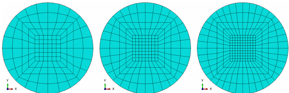
Fig. 8 132, 192, and 260 Q9 meshes used for the circular plate
