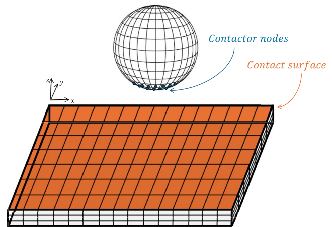
Fig. 3 Node-to-surface contact method
