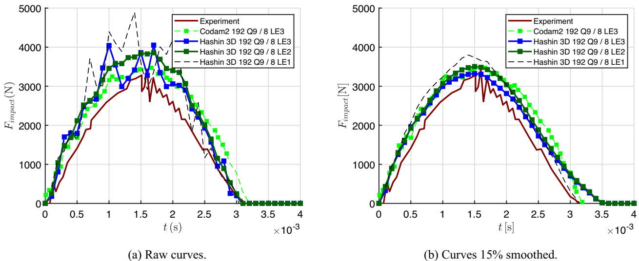
Fig. 10 Effect of through-thickness expansion order of the impact force-time response for the circular composite plate. Experimental results are from [8], CODAM2 reference results are from [13]
