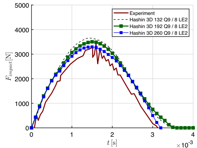
Fig. 9 In-plane mesh refinement effect of the impact force-time response for the circular composite plate with 15% smoothing. Experimental results are from [8]
