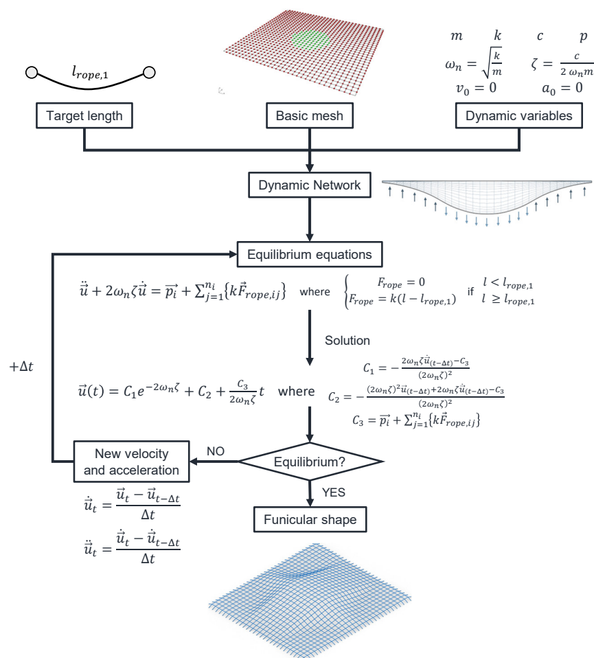
Figure 3. MRA workflow.
