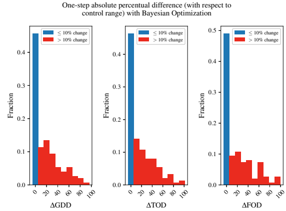
Figure 2: One-step absolute percentage change in control parameters with respect to physical control range ( 100 \cdot \frac{|\psi_i(k) - \psi_i(k-1)|}{\psi_i^{\max} - \psi_i^{\min}} ). Plots are specific to the actual control parameter. One-step percentage differences that are over 10% are colored in red.
