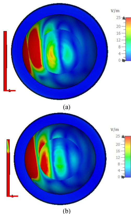
Figure 3. Simulated electromagnetic response of the proposed antenna: (a) electric-field distribution inside the phantom-loaded model at 0^\circ , (b) electric-field distribution inside the phantom-loaded model at 90^\circ .
