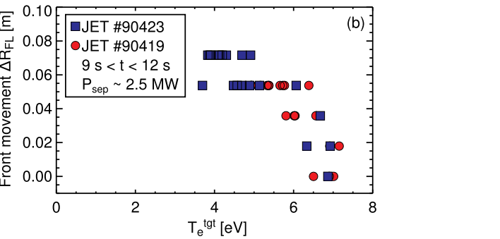
Fig. 6. Spectroscopic measurements of c_N and the amount of movement of the N II emission front away from the strike point are shown as a function of the strike point temperature from Langmuir probes for two JET L-mode plasma in (a) and (b), respectively. Scaling law predictions of c_N required for detachment are indicated in (b) by the dashed lines for two values of f_{GW, sep} .
