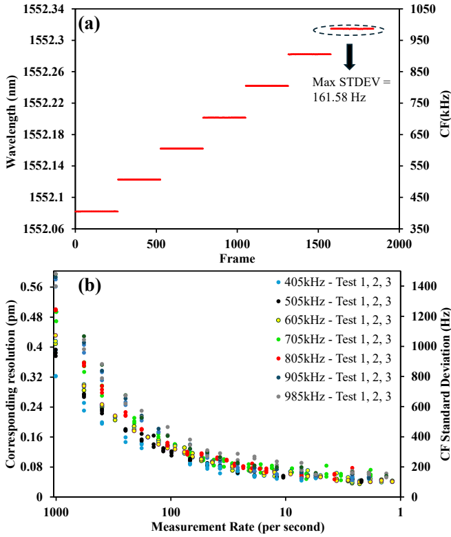
Fig. 8. Static FBG interrogation results (a) Estimated CF for different Bragg-wavelength settings, and (b) \sigma of the estimated CF across different Bragg wavelengths and measurement rates.
