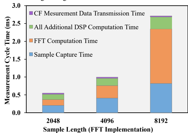
Fig. 4. Cumulative/total processing times for the CF measurement process, with no DFT averaging. Not shown in figure, 16384 FFT yields a total CF measurement processing time of \sim 9.3 ms, of which the sample capture time accounts for 1.638 ms, FFT computation time accounts for 7.030 ms, and all Additional DSP Computation Time accounts for 0.579 ms. CF: centre frequency, DFT: discrete Fourier transform, FFT: fast Fourier transform.
