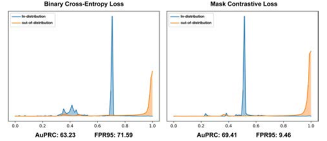
Fig. 14. Outlier Loss Comparison : During the training Mask2Anomaly, on the outlier set, we find that incorporating a mask contrastive loss, which is a margin-based loss function, resulted in better performance compared to the conventional binary cross-entropy loss. These experiments were conducted on the FS L&F validation set.
