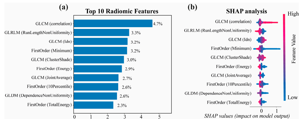
Figure 5. SHAP-based explainability analysis of the radiomic model. (a) Ranking of the top 10 radiomic features based on mean absolute SHAP values. (b) SHAP summary plot illustrating the magnitude and direction of feature effects across ROIs in the test set.
