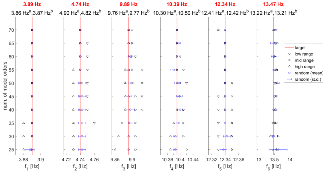
Figure 3: Estimated natural frequencies for the MC Sampling AOMA procedure, in comparison with the range-reduced deterministic alternatives and the target values (full-range deterministic AOMA).
