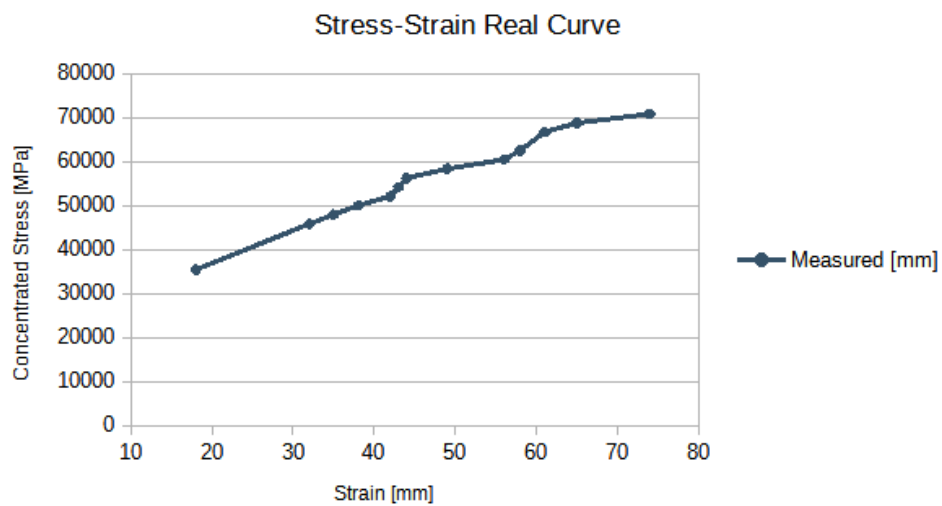
Figure 4: Load displacement behaviour of the vault
