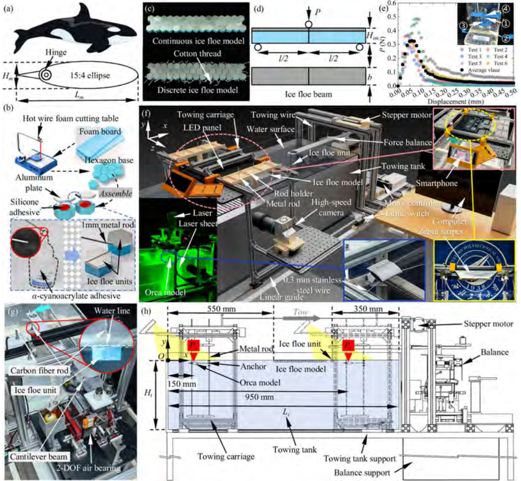
Figure 2. (a) Comparison between real orca morphology and simplified orca model. (b) Fabrication of ice floe unit. (c) The continuous and the discrete ice floe model. (d) Schematic diagram of the three-point bending test for ice floe beams. (e) Three-Point Bending Test. (f) Experimental towing tank and related arrangements. (g) The three-dimensional micro-force measurement balance. (h) The side view of the towing tank clearly illustrates the installation relationships of the measurement devices and multiple critical dimensions. The edge of the upstream water surface in the towing tank is regarded as the geometric origin for describing key locations in the side view.
