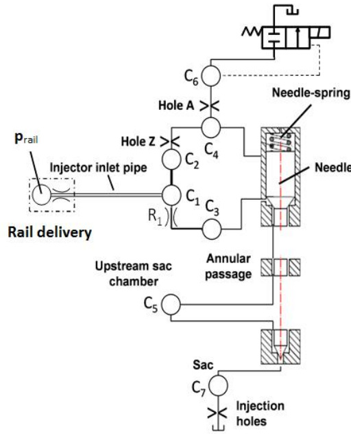
Figure 7. Schematic of the 1D hydraulic-mechanical- numerical model.
