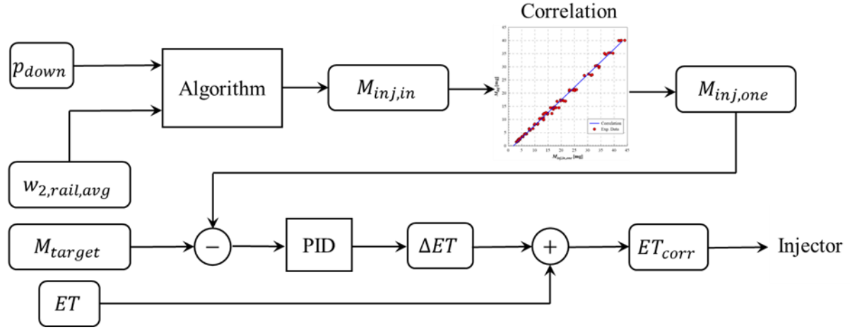
Figure 18. Example of a possible closed-loop control strategy for the ET correction.
