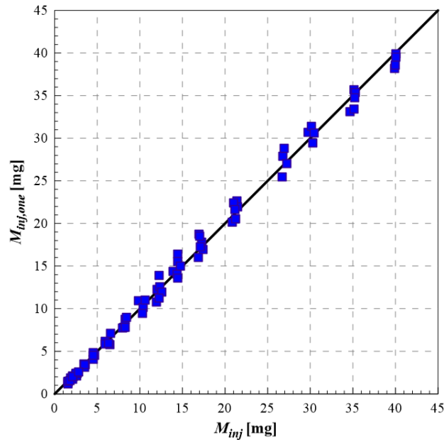
Figure 16. Prediction performance of the M_{inj} vs M_{inj,in,one} correlation.
