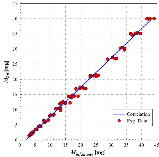
Figure 15. Correlation between M_{inj} and M_{inj,in,one} for evaluation method employing one sensor.
