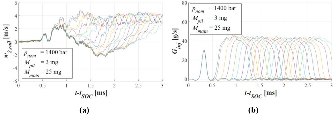
Figure 17. Time distributions of w_{2,rail} and G_{inj} for pilot-main injections with different DT values: (a) w_{2,rail} ; (b) G_{inj} .
