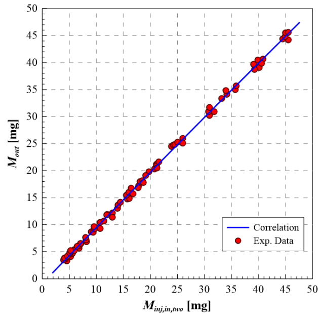
Figure 6. Correlation between the mass entering the injection and the outlet one.
