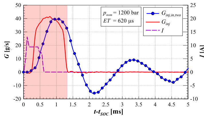
Figure 3. Flow-rate entering the injector, injected flow-rate and current signal.
