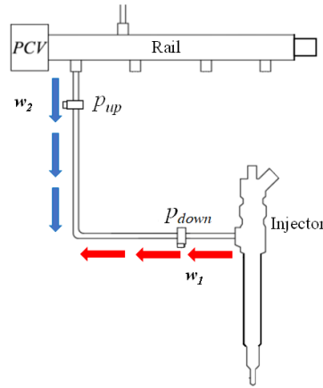
Figure 9. Schematic of elementary waves.
