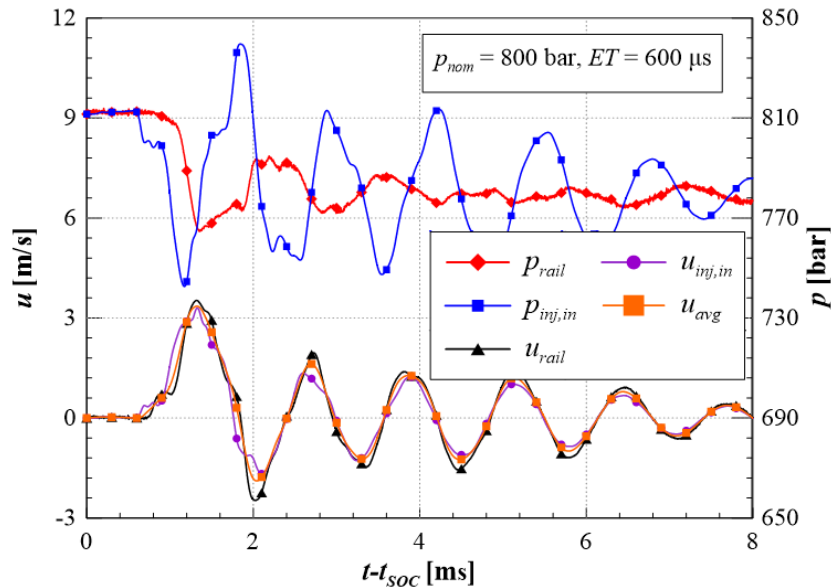
Figure 12. Time histories of the flow velocities at the extremities of pipe feeding the injector.
