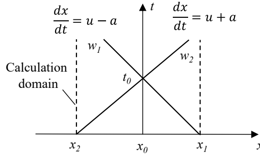
Figure 8. Characteristic curves for the tube model.
