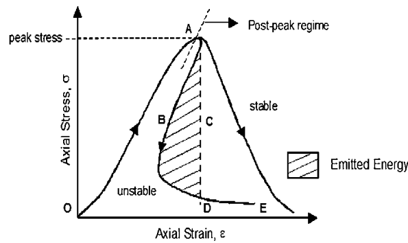
Fig.1. Stable and catastrophic (snap-back) response (modified from Lacidogna et al. , 2019)
