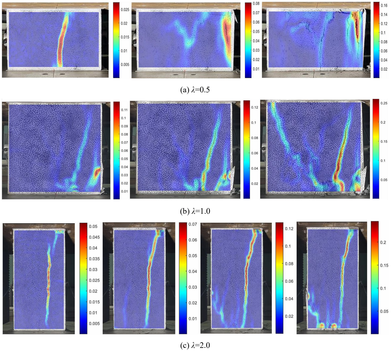
Fig.11. DIC strain cloud diagram of the fracture process in concrete specimens with size equal to 300 mm and slenderness equal to (a) \lambda = 0.5 , (b) \lambda = 1.0 , and (c) \lambda = 2.0 .
