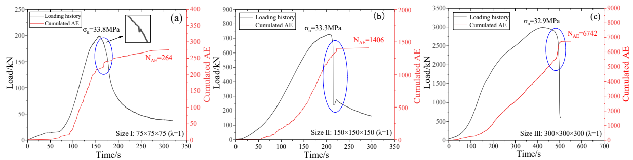
Fig.9. Loading history and cumulated AE curve for concrete specimens with slenderness equal to 1 and size of (a) 75 mm, (b) 150 mm, and (c) 300 mm. A correlation emerges between loading drops (snap-back instabilities) and AE jumps (emitted energy, E).
