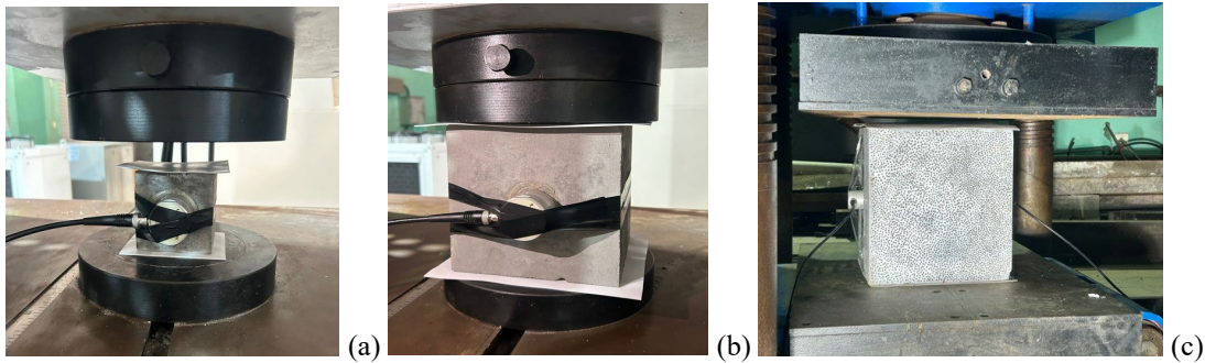
Fig.8. Loading layouts for specimens with slenderness equal to 1 and size of (a) 75 mm, (b) 150 mm, and (c) 300 mm.
