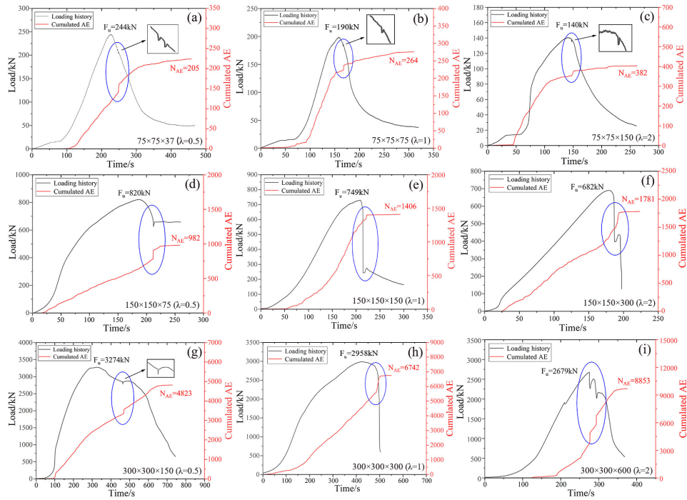
Fig.12. Loading history and cumulated AE curve for different specimen volumes with slenderness equal to 0.5, 1.0, and 2.0, and sizes of 75, 150, and 300 mm.
