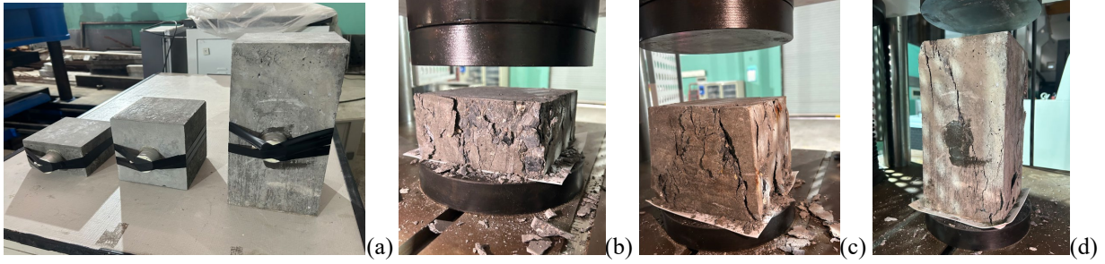
Fig.6. Final collapse for concrete specimens (a) with size of 150 mm, and slenderness (b) \lambda = 0.5 , (c) \lambda = 1.0 , and (d) \lambda = 2.0 .
