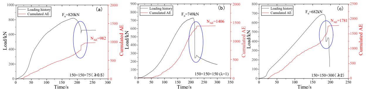
Fig.7. Loading history and cumulated AE curve for concrete specimens with slenderness equal to (a) \lambda = 0.5 , (b) \lambda = 1 , and (c) \lambda = 2.0 , and size of 150 mm. A correlation emerges between loading drops (snap-back instabilities) and AE jumps (emitted energy, E).
