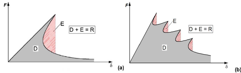
Fig.2. Load-displacement curves representing: (a) a catastrophic behaviour (single snap-back); (b) a global softening behaviour perturbed by multiple local instabilities (snap-back) (modified from Carpinteri et al. , 2018).
