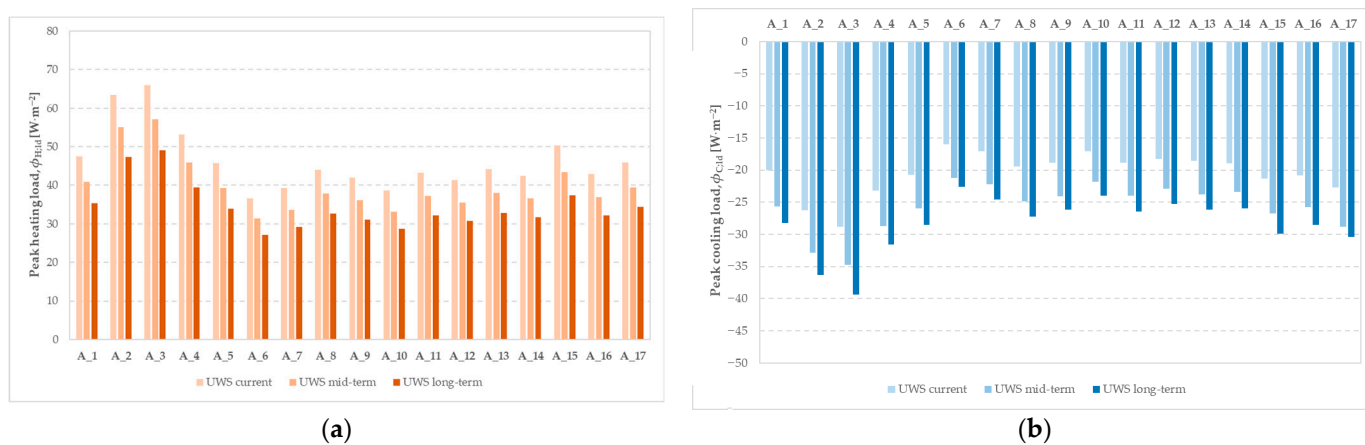
Figure 8. Peak heating (a) and cooling (b) loads using UWS data for the current, mid-, and long-term periods.
