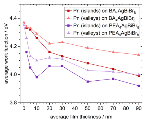
Figure 5. Work function depending on the average film thickness of Pn on \text{BA}_4\text{AgBiBr}_8 or \text{PEA}_4\text{AgBiBr}_8 found on top of Pn islands or in valleys between Pn islands.
