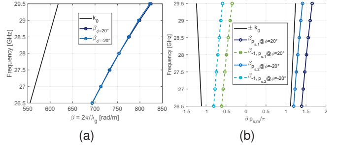
Fig. 2. (a) Dispersion diagram for sectorial waveguide with concentric radial glide-symmetric corrugations at \phi = \pm 20^\circ . (b) Normalized (respect the slot period p_{s,m} ) dispersion diagrams for the radial glide-symmetric corrugated sectorial waveguide at \phi = 20^\circ with p_{s,1} = 6.3 mm and \phi = -20^\circ and p_{s,2} = 5.4 mm. The curves are obtained by (1a) and the results in Fig. 2a. Fundamental harmonic \beta (solid dark blue line) and visible harmonic \beta_{-1} (dashed green line) at \phi = 20^\circ with p_{s,1} = 6.3 mm. Fundamental harmonic \beta (solid light blue line) and visible harmonic \beta_{-1} (dashed light blue line) at \phi = -20^\circ with p_{s,2} = 5.4 mm. Lines of the light \pm k_0 (black lines).
