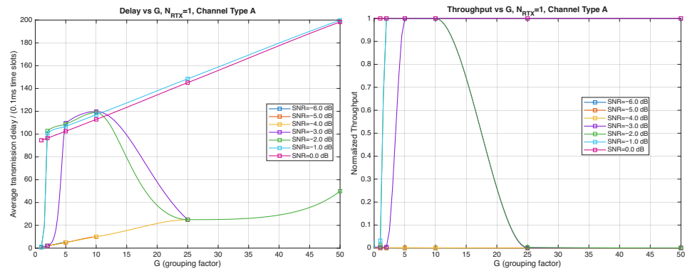
Figure 20. Average transmission delay of successful packets and normalized throughput with HARQ-II versus G for N_{RTX} = 1 (Channel type A, \mu = 0, R_c = \frac{1}{2}, N_{\Delta} = 100 , very low SNR).
