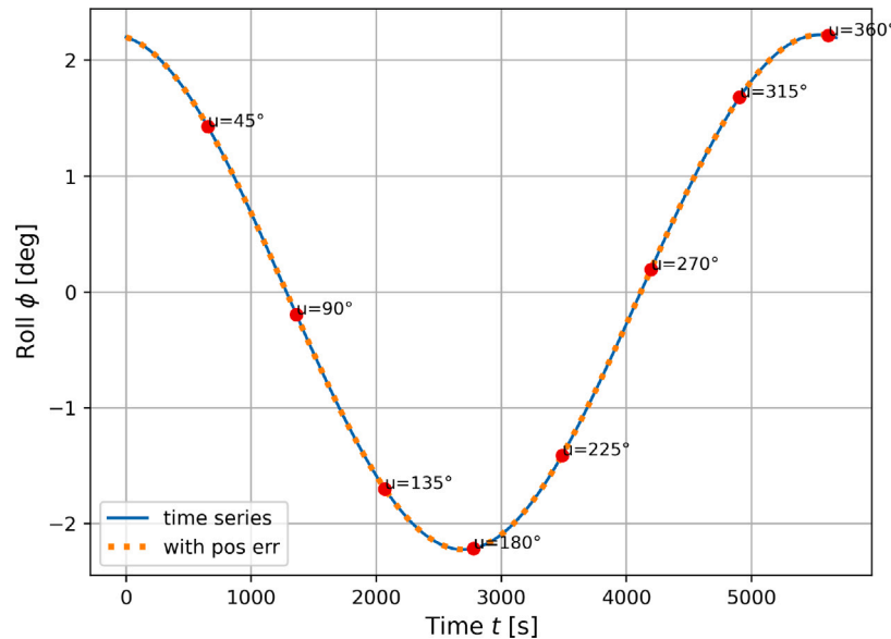
Fig. 14. Roll time series (in blue) and its profile in case of a forward in-track position error of 2 km (orange dashed). The red dots highlight the roll angle at specific arguments of latitude of INCUS 1.
