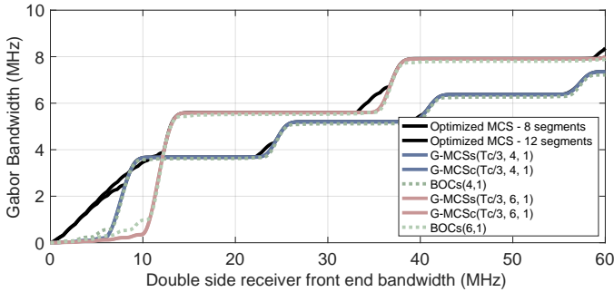
(a) Even number of subchips.
