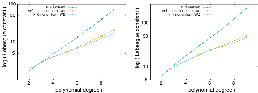
Fig. 7 In 3D, the Lebesgue constant in semi-log scale as a function of the polynomial degree r \geq 2 of the k -form in a tetrahedron T with k = 0 (left) and k = 1 (right), respectively
