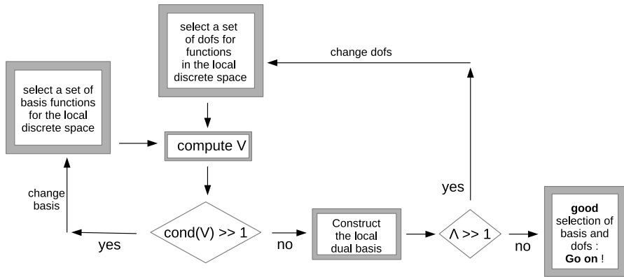
Fig. 1 Simplified visualization of the interaction among decisive ingredients or steps for the success of the multivariate high-order polynomial approximation. The conditioning of the Vandermonde matrix V matters when computing the dual basis and the growth of the Lebesgue constant \Lambda with the approximation degree r has to be slow for a stable interpolation
