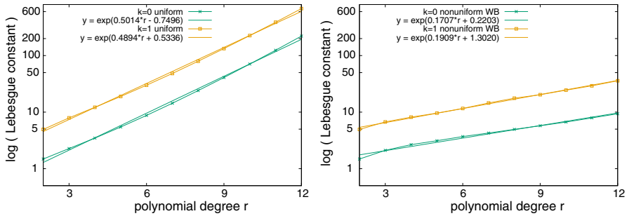
Fig. 6 In 2D, the Lebesgue constant in semi-log scale as a function of the polynomial degree r \geq 2 of the k -form in a triangle T , uniform case (left) and nonuniform case (right), together with their fittings, respectively
