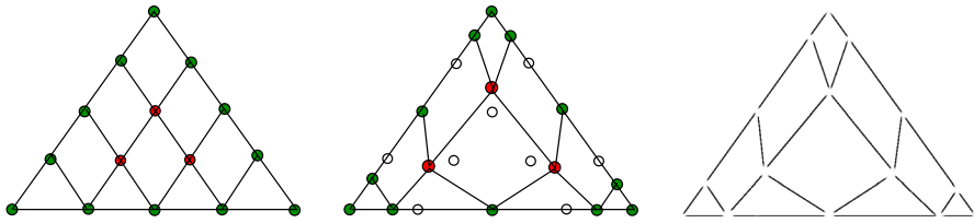
Fig. 4 Construction, in a triangle F , of a nonuniform distribution of small edges that are \perp to the edges E of F , with ending points in either the symmetrised Lobatto or warp & blend nodes (here drawn for the scalar interpolation of degree r = 4 ). On the left, the uniform set of points and edges; at the center, points on edges and at the interior are moved in new positions thus defining the new set X_r^0(F) ; on the right, the resulting set X_r^1(F) of small edges in F
