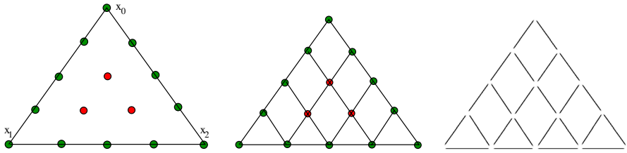
Fig. 2 Construction, in a triangle F , of a uniform and parallel distribution of small edges with ending points in the nodes of the principal lattice (here drawn for r = 4 ). On the left, the points of the principal lattice X_r^0(F) ; on the right, the set of edges X_r^1(F)
