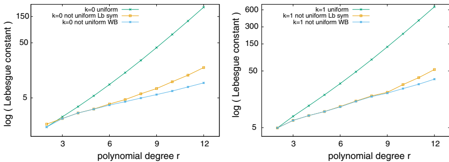
Fig. 5 In 2D, the Lebesgue constant in semi-log scale as a function of the polynomial degree r \geq 2 of the k -form in a triangle T , with k = 0 (left) and k = 1 (right), respectively
