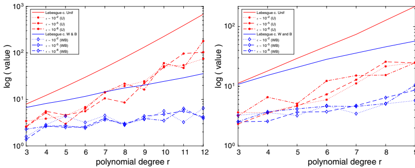
Fig. 9 Comparison between the estimated Lebesgue constants (straight lines) and the numerical ones, computed through the stability test (non-continuous lines) for small edges associated with uniform (red) and warp & blend (blue) node distributions, in 2D (left) and 3D (right)
