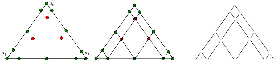
Fig. 3 Construction, in a triangle F , of a nonuniform distribution of small edges that are \parallel to E \in \Delta_1(T) , with ending points in the Lobatto nodes (here drawn for r = 4 ). On the left, the set of points X_r^0(F) ; on the right, the set of edges X_r^1(F)
