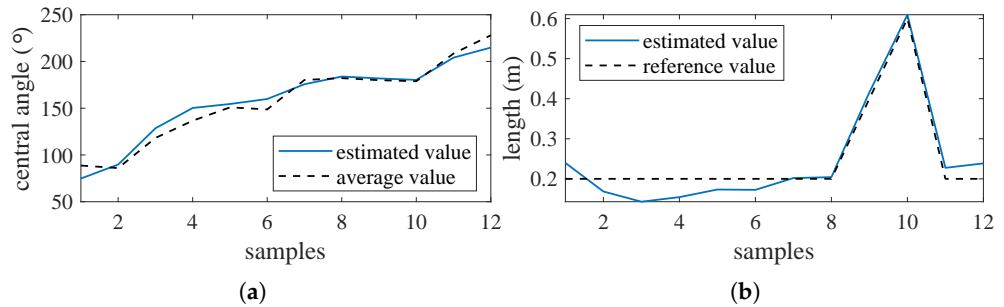
Figure 10. Size evaluation of irregular shield holes. (a) The estimated results of defect angles; (b) the estimated results of defect lengths.
