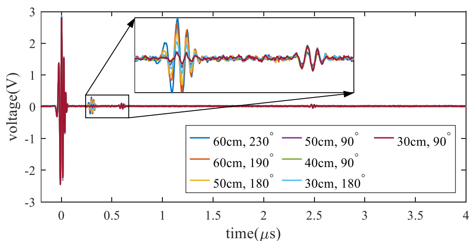
Figure 14. Reflected signals from cable with two shield hole defects.
