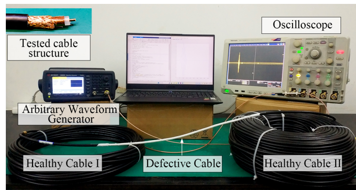
Figure 11. Experiment setup.
