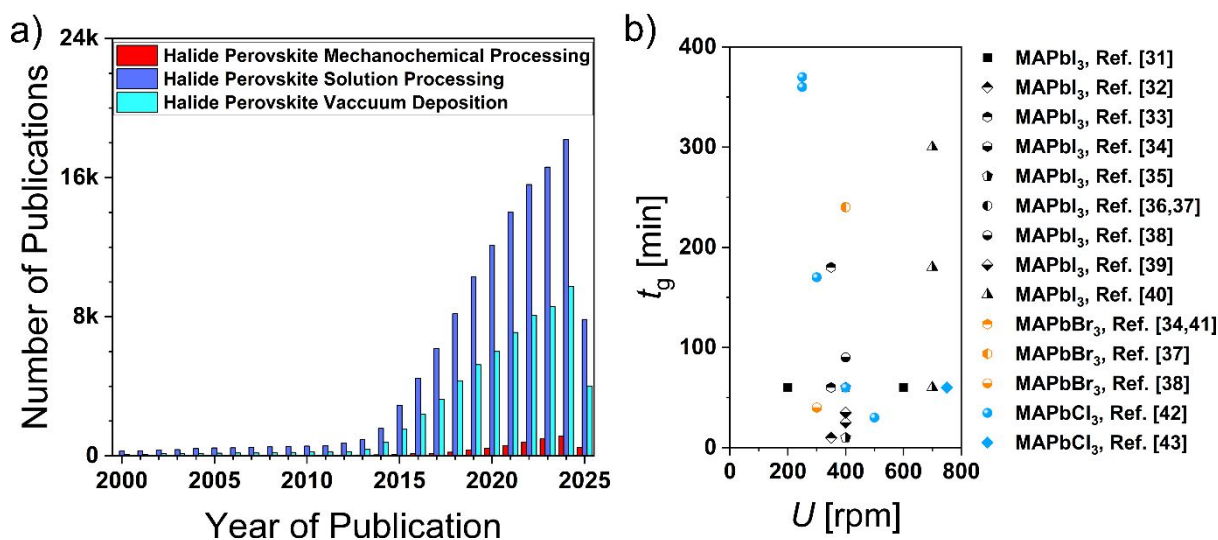
Fig. 1: a) Number of publications on halide perovskites synthesised via mechanochemical, solution and vacuum processing from 2000 to 2025 obtained using Google Scholar. b) Total grinding time ( t_g ) and rotation speed ( U ) reported in the literature for methylammonium lead halide (MAPbX 3 ) perovskites.
