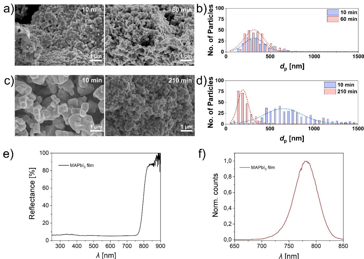
Fig. 4: a) Top-SEM images and b) particle size distributions of MAPbI 3 powder ground at 400 rpm with a BTR of 20:1. c) Top-SEM images and d) particle size distributions of MAPbI 3 powder ground at 800 rpm with a BTR of 8.5:1. e) Reflectance and f) photoluminescence spectra of MAPbI 3 film coated on FTO. The energy gap, estimated by the maximum peak of the PL, is 1.59 eV.
