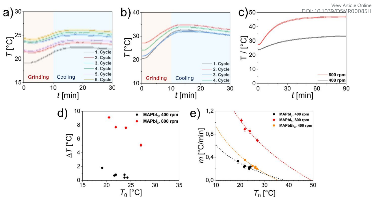
Fig. 3: a) Lid temperature profile of MAPbI 3 mechanochemical synthesis for cycles of 10 minutes of grinding followed by 20-minute breaks at 400 rpm and b) 800 rpm employing a BTR of 8.6:1. c) Lid temperature profile of MAPbI 3 mechanochemical synthesis measured during continuous grinding for 90 minutes at 400 rpm and 800 rpm with a BTR of 8.6:1. The shaded error bands reflect error bars due to the inaccuracy of the thermal sensor of \pm 1\% . d) Evolution of the lid temperature difference ( \Delta T ) developed within the first 8.5 min of grinding as a function of the initial temperature ( T_0 ). e) Slope ( m ) of the temperature profile plotted as a function of the initial temperature for MAPbI 3 ground at 400 and 800 rpm and MAPbBr 3 ground at 400 rpm and exponential fit. The linear fittings of the temperature profiles are shown in Fig S4. Exponential fitting parameters are listed in Table S2.
