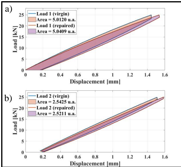
Figure 5: Load-displacement response and area for the Load 1 (a) and Load 2 (b) steps. (u.a. = unity of area).
