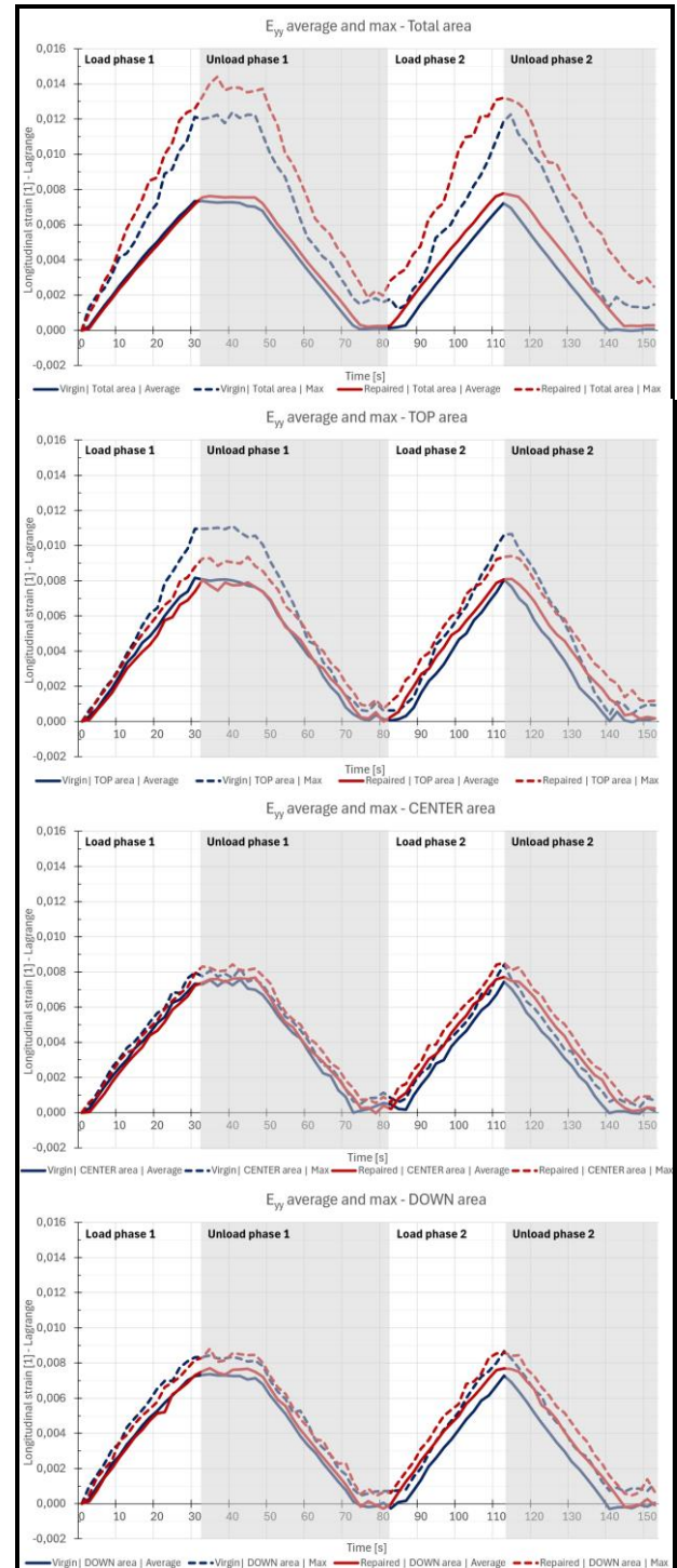
Figure 10: Longitudinal strain ( E_{yy} ) value over time, from top to bottom respectively total area of interest, top area, center area, down area.
