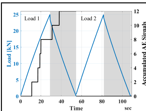
Figure 6: Accumulated AE Signals for the virgin sample.
