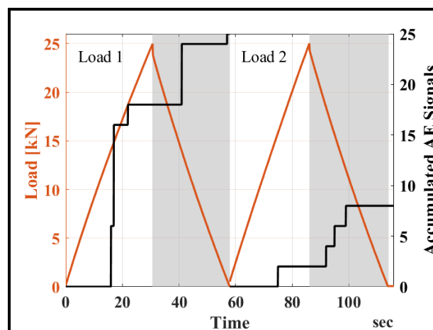
Figure 7: Accumulated AE signals for the repaired sample.
