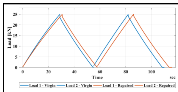
Figure 3: Load - time of the tensile test.
