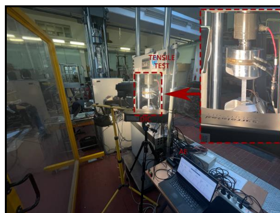
Figure 2: Detail of test setup and apparatus.
