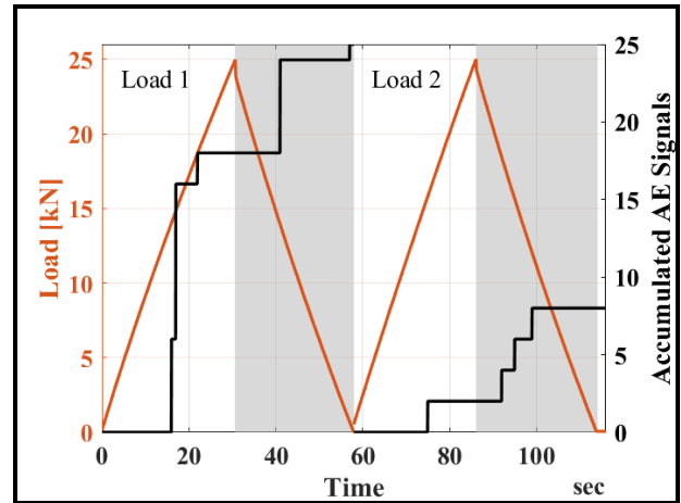
Figure 7: Accumulated AE signals for the repaired sample.
