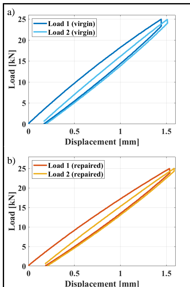
Figure 4: Load-displacement response from the tensile test for the virgin (a) and repaired (b) versions.
