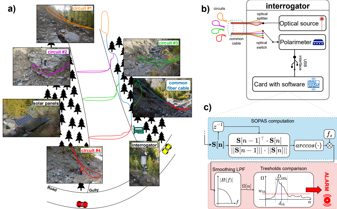
Fig. 1. (a) Experimental setup of the monitored gully, including photos of the actual fiber installations, interrogator, and solar panels. Red, green, purple, yellow, and blue lines refer to circuits #4, #3, #2, #1, and common fiber cable. (b) Simplified interrogator scheme. (c) Proposed processing and alarming algorithm running in the card connected to the polarimeter.
