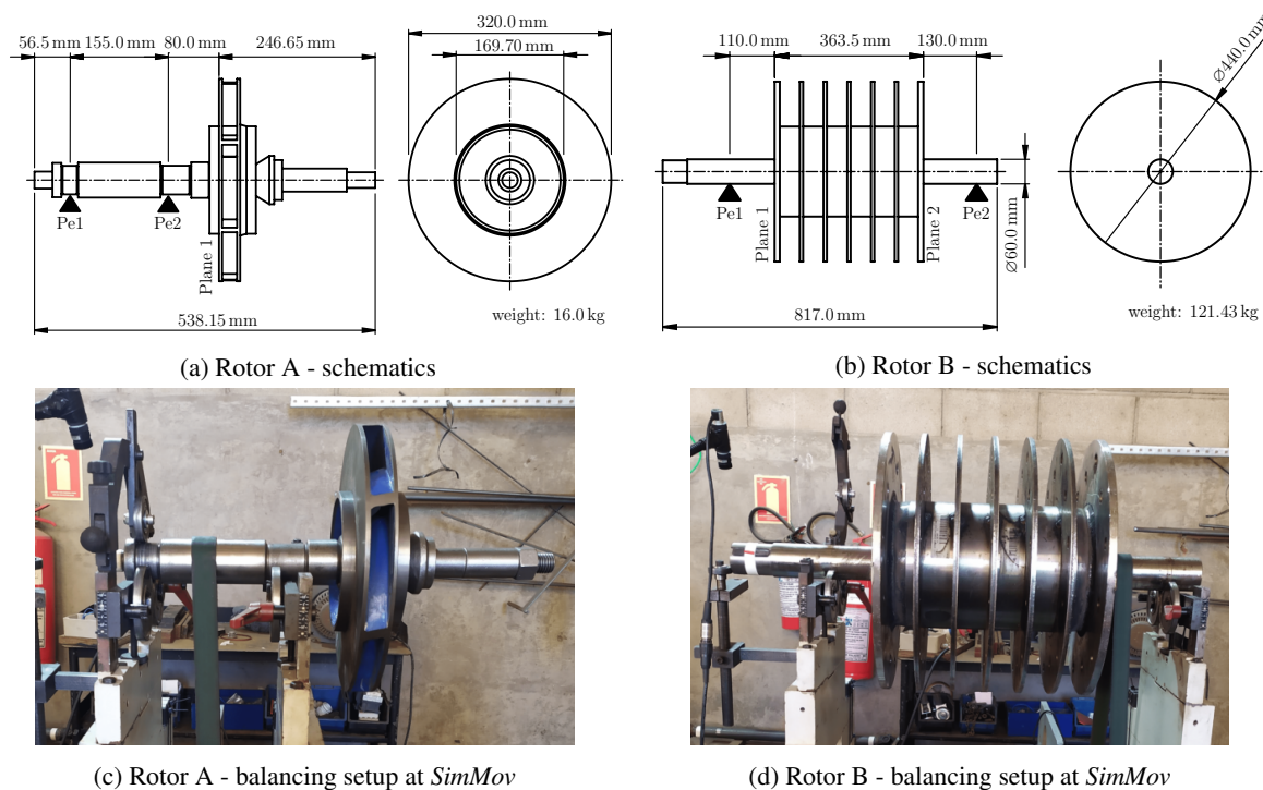
Figure 2. Rotors balancing being conducted using unconventional machinery: SimMov
