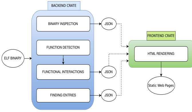
Fig. 1. Architecture and components interactions of the manifest-producer
