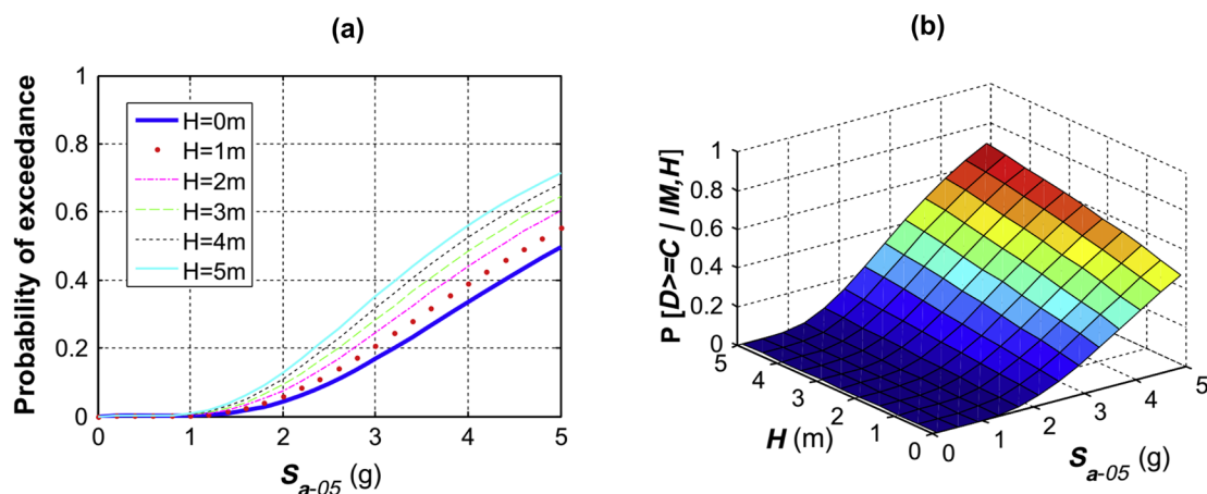
Figure 1. (a) Fragility curves and (b) fragility surface of a short-span bridge under combined scour and seismic hazard. The intensity measure is the spectral acceleration at a period of 0,5s S_{a-0.5} (from Wang et al. , 2014b).
