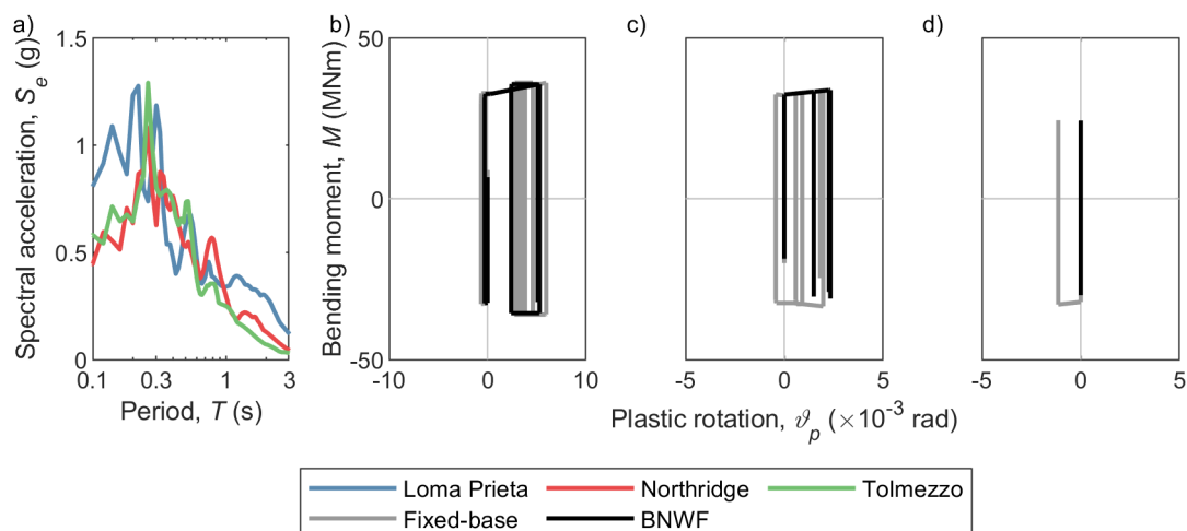
Figure 4. a) Response spectra of the considered input motions; b-d) Moment vs. plastic rotation of the pier for the Loma Prieta (b), Northridge (c), and Tolmezzo (d) motions.
