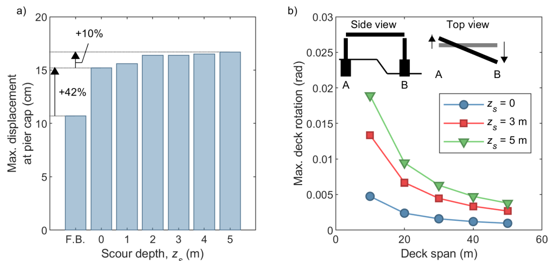
Figure 6. a) Maximum displacement at the pier cap for the fixed-base model (F.B.) and as a function of the scour depth; b) Maximum deck rotation as a function of the span length and the scour depth, under the assumption of deck supported by a scoured pier and an unscoured pier.
