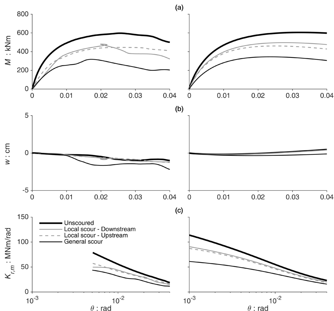
Figure 9. Experimental results (left) compared to numerical predictions (right): (a) moment-rotation; (b) settlement-rotation; and secant rocking stiffness-rotation response (from Ciancimino, Anastasopoulos, et al. 2022).
