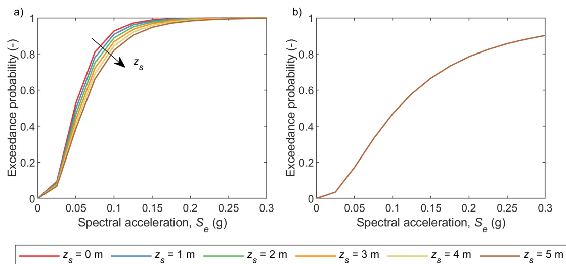
Figure 5. Fragility curves as a function of the scour depth z_s , for a) moderate damage stage and b) severe damage state.
