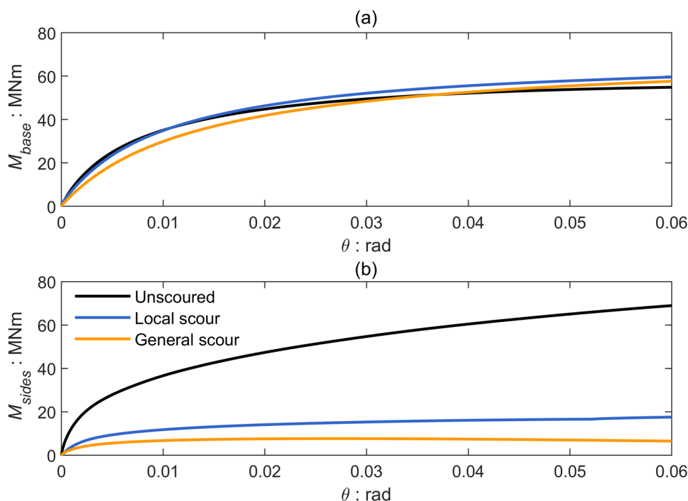
Figure 11. Resisting moment exerted by bearing capacity mechanism (a) and by the soil thrusts along the sides of the footing (b).
