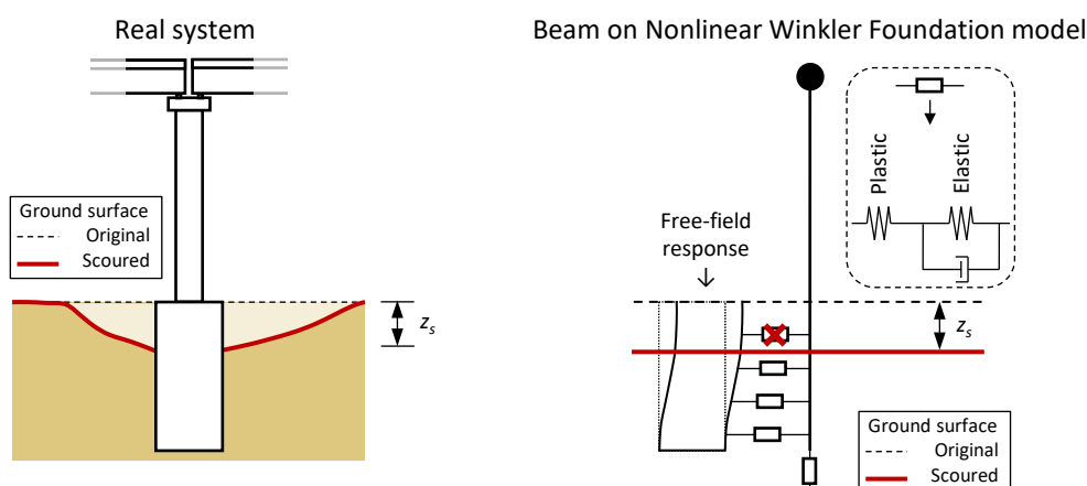
Figure 3. Real system vs. Beam on nonlinear Winkler foundation model.
