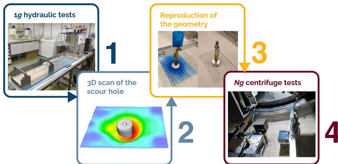
Figure 8. Experimental methodology: (1) development of the scour hole through the MTG; (2) 3D scanning of the scour hole; (3) reproduction of the scour hole geometry; and (4) study of the mechanical part of the problem through centrifuge model testing.
