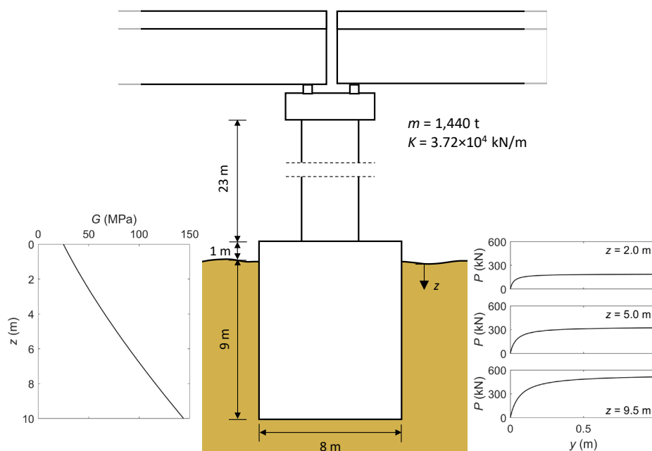
Figure 2. Case study with main information about geometry, structural and soil parameters. Description of soil behaviour is provided both in terms of G profile and p - y curves at different depths.
