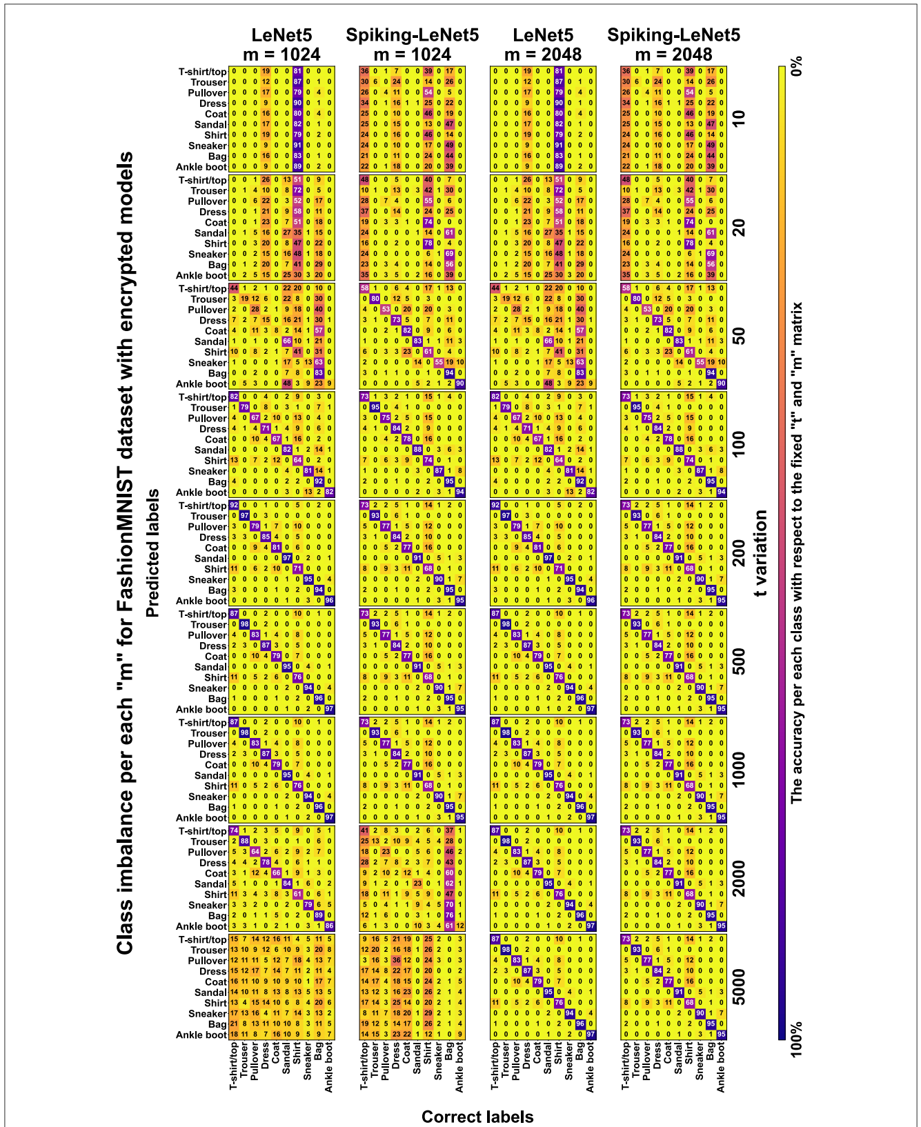
FIGURE 19 Encrypted confusion matrix for FashionMNIST with t and m variation. It can be noticed that for low values of t , the results tend to concentrate on labels that resemble each other the most. Spiking-LeNet5 is less random than LeNet5 for low values of t .
