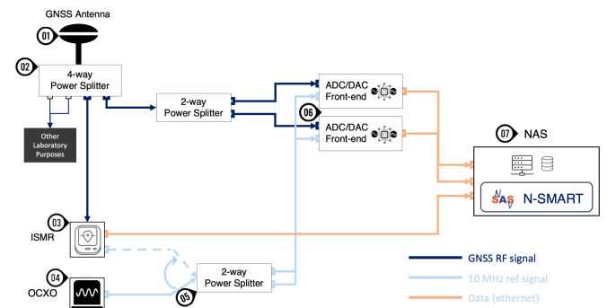
Fig. 3: Hardware scheme.
