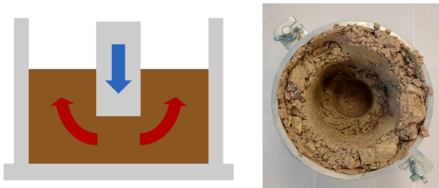
Fig. 5. Scheme of the soil flow under the blow of the Proctor ramming weight (left); Instance of failure of the Proctor test (right).
