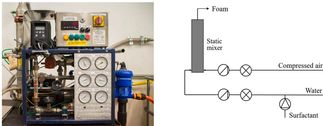
Fig. 4. Left: Foam generator picture. Right: Foam generator scheme. The generator operates with a maximum liquid flow of 11.9 l/min and a maximum air pressure of 4 bar, with both flow rates finely regulated through needle valves. The static mixer with specific dimensions, including an internal diameter ( D_i ) of 78 mm, a length ( L ) of 450 mm, and it is filled with glass fragments with a mean diameter of 5 mm. The volumetric pump for surfactant is equipped with a mixing chamber to ensure a correct mixing of water and surfactant.
