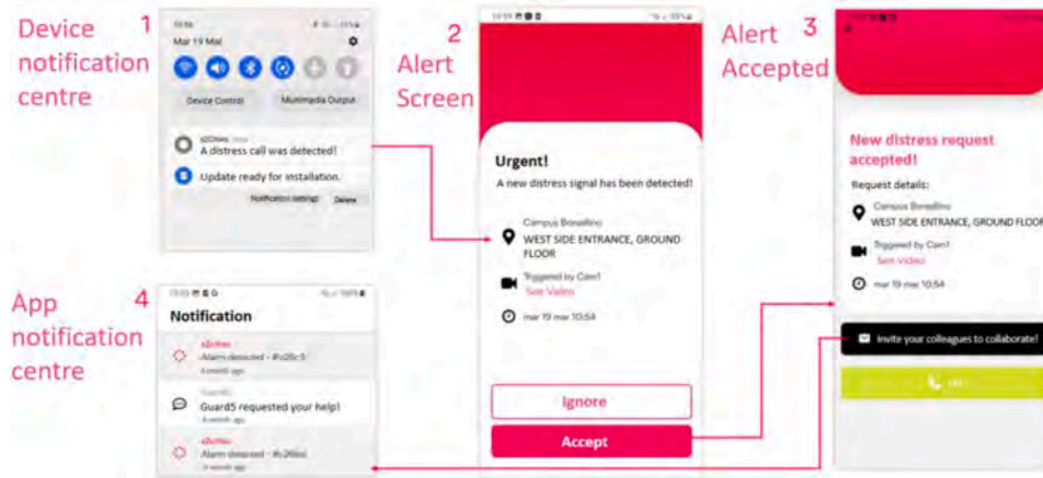
Fig. 11. Workflow of the real-time alert system, from notification delivery to alert acceptance, including event details and user actions.
