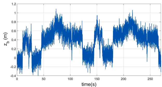
Fig. 3. Example of raw barometric signal, converted to altitude, recorded during one of the experimental sessions.
