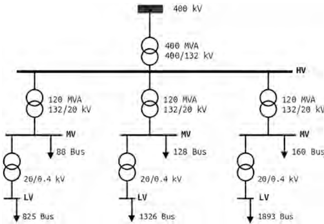
Fig. 8. Arbarello substation electrical schema.
