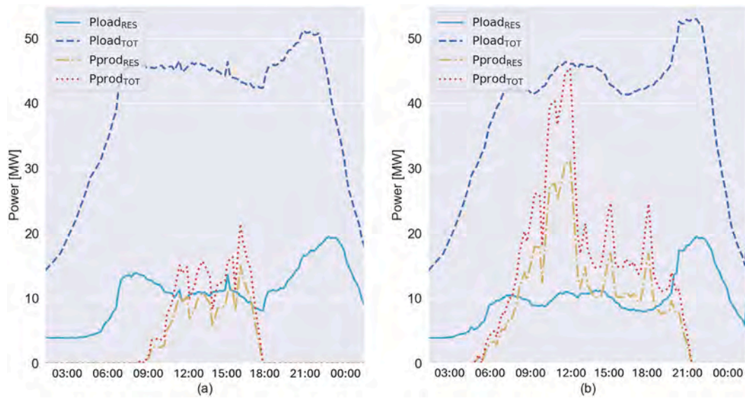
Fig. 11. Daily power flows for Arbarello substation: daily consumed power with residential buildings only ( P_{load\_RES} ) (MW), daily consumed power with all buildings (i.e., residential, commercial and industrial) ( P_{load\_TOT} ) (MW), daily produced power with residential buildings only ( P_{prod\_RES} ) (MW) and daily produced power with all buildings (i.e., residential, commercial and industrial) ( P_{prod\_TOT} ) (MW).
