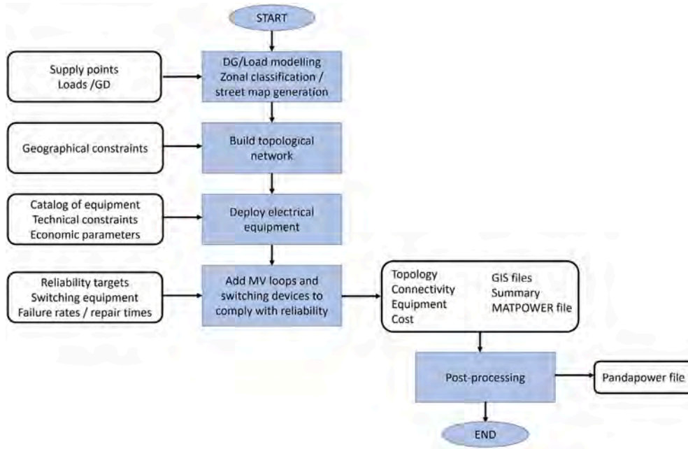
Fig. 2. Logical architecture of the Reference Network Model: steps involved and relevant input and output data.
