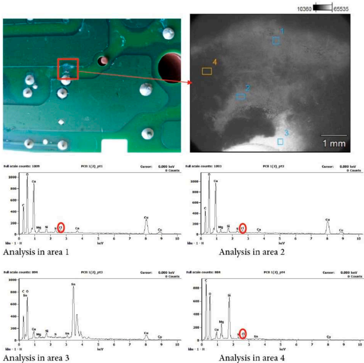
Fig. 2. FE-SEM analysis of the PCBA under test.
