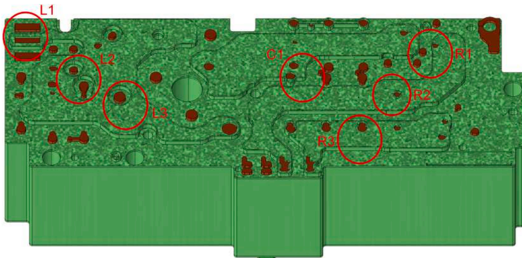
Fig. 5. Pinhole created in the solder mask, exposing the underlying copper (located on the edge of the track).
