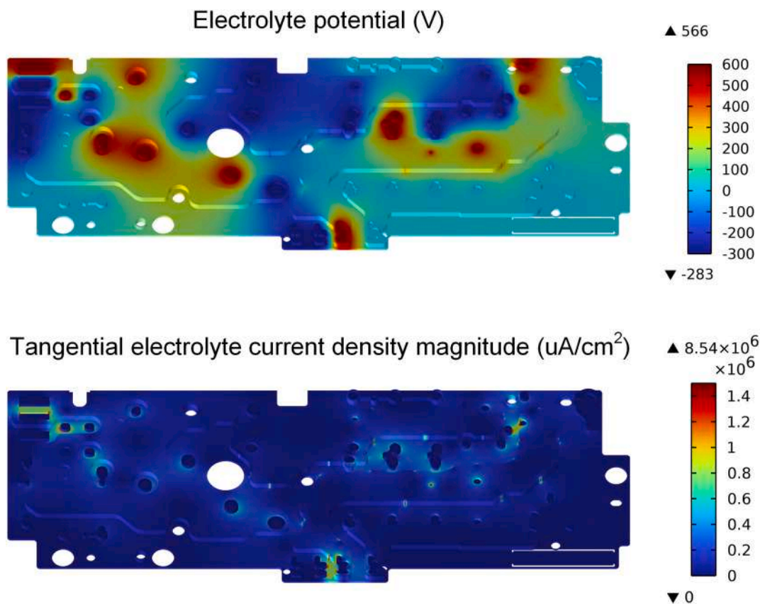
Fig. 12. Electrolyte potential and current density distributions on the PCB surface (with pinholes).
