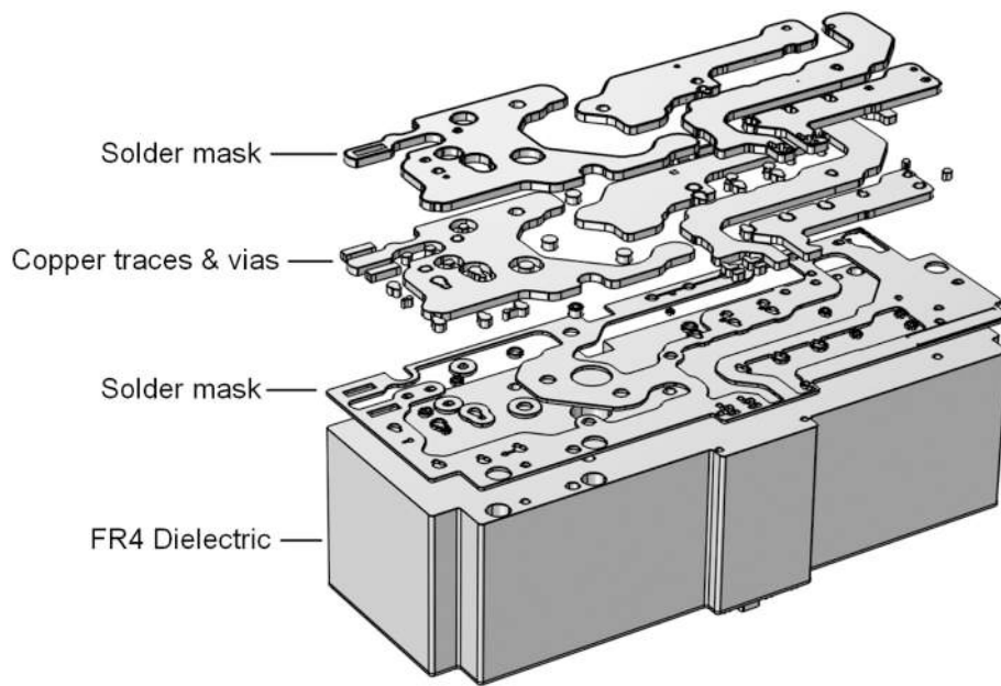
Fig. 3. Cross-section and top view of solder masks represented in the numerical model.
