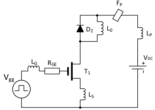
(a) Double-pulse test circuit.
