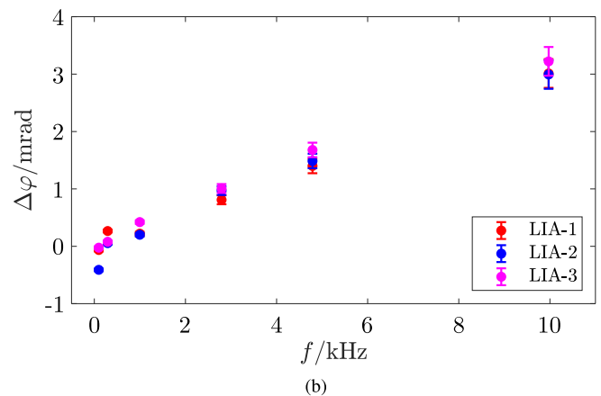
Fig. 3. Comparison of the magnitude and phase calibration of LIA-1 (red), LIA-2 (blue) and LIA-3 (magenta) with |V_{\text{CAL}}^{\text{nom}}| = 5 \mu\text{V} , \varphi_{\text{CAL}}^{\text{nom}} = 45^\circ , and n = 8 , as a function of f_{\text{CAL}} ; LIAs set as per Table III. Uncertainty bars represent combined standard uncertainty. (a) Magnitude error \delta R as a function of f_{\text{CAL}} . (b) Phase error \Delta\varphi as a function of f_{\text{CAL}} .
