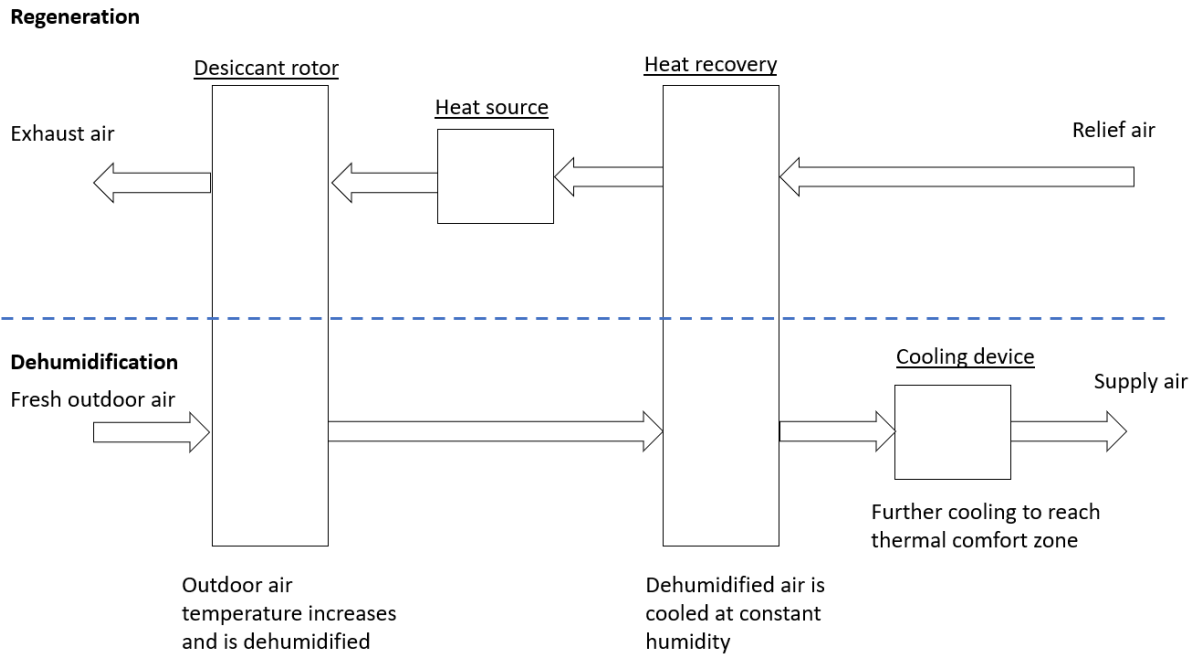
Figure 22: Simplified schematic representation of desiccant dehumidification.
