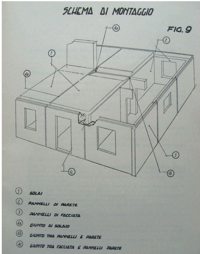
Fig. 6. Baretts system, general assembly scheme of the elements. Source: GescaI, IACP Turin, 1966.
