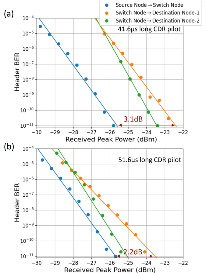
Fig. 9. Header BER measured at QWSR at the core (blue traces) and at the edges (orange and green traces) vs. received peak power for (a) 41.6 \mu\text{s} and (b) 51.6 \mu\text{s} long CDR pilot sequence.
