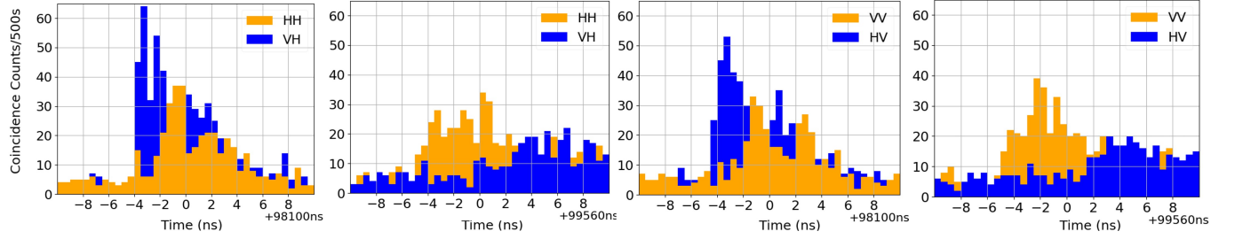
Fig. 4. Coincidence counts distributions, first-row plots with narrow-band photon pairs (1574, 1557.51) nm, second-row plots with broadband photon pairs. The first and third column plots represent destination-2 measurements, around 98100 ns delay. The second and fourth column plots represent destination-1 measurements, around 99560 ns delay.
