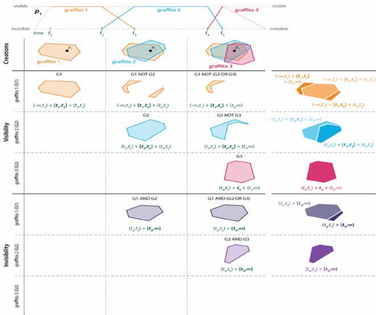
Figure 5. When polygons represent graffiti, tracking which part(s) of each graffiti become(s) invisible over time becomes possible. Every derived polygon comes with two pieces of information. Above each polygon, one finds the boolean algebra used in its computation. The mathematical formulation below each polygon represents the certain and fuzzy portions of its visibilityspan.
