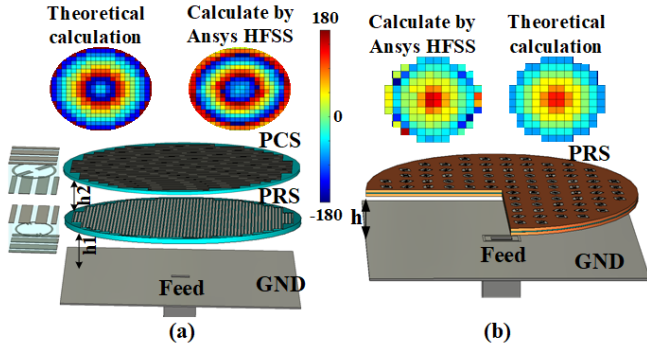
Fig. 3. The concerned non-resonant PRSA configurations and the phase distributions on the bottom surfaces of the PRS: (a) with separate PRS and PCS; (b) with a single superstrate combining the functionalities of the PRS and PCS.
