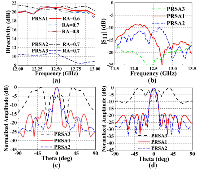
Fig. 4. The simulated results for PRSA1, PRSA2, and PRSA3: (a) directivities, where RA denotes the uniform reflection amplitude of the PRS; (b) |S_{11}| ; (c) radiation patterns at 12.5 GHz in the E plane; (d) radiation patterns at 12.5 GHz in the H plane.
