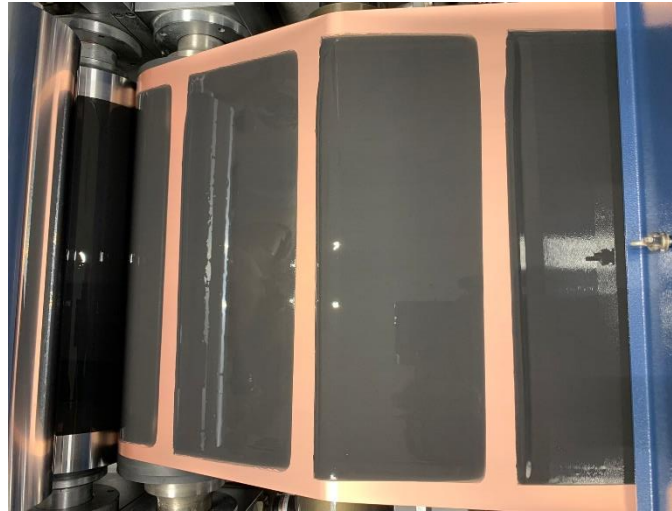
Figure 1. Anode coating on roll-to-roll machine
