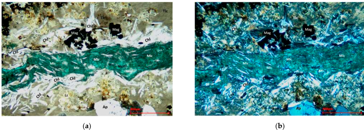
Figure 6. Optical microscopy thin section images in parallel transmitted light (PL) and cross-polarized transmitted light (XPL): (a) thin section nr. 3 in PL; (b) thin section nr. 3 in XPL. Identified minerals: Ap—apatite, Mag—magnetite, Tlc—talc, Chl—chlorite, Lz—lizardite, Mlc—malachite (abbreviation according to [43]).
